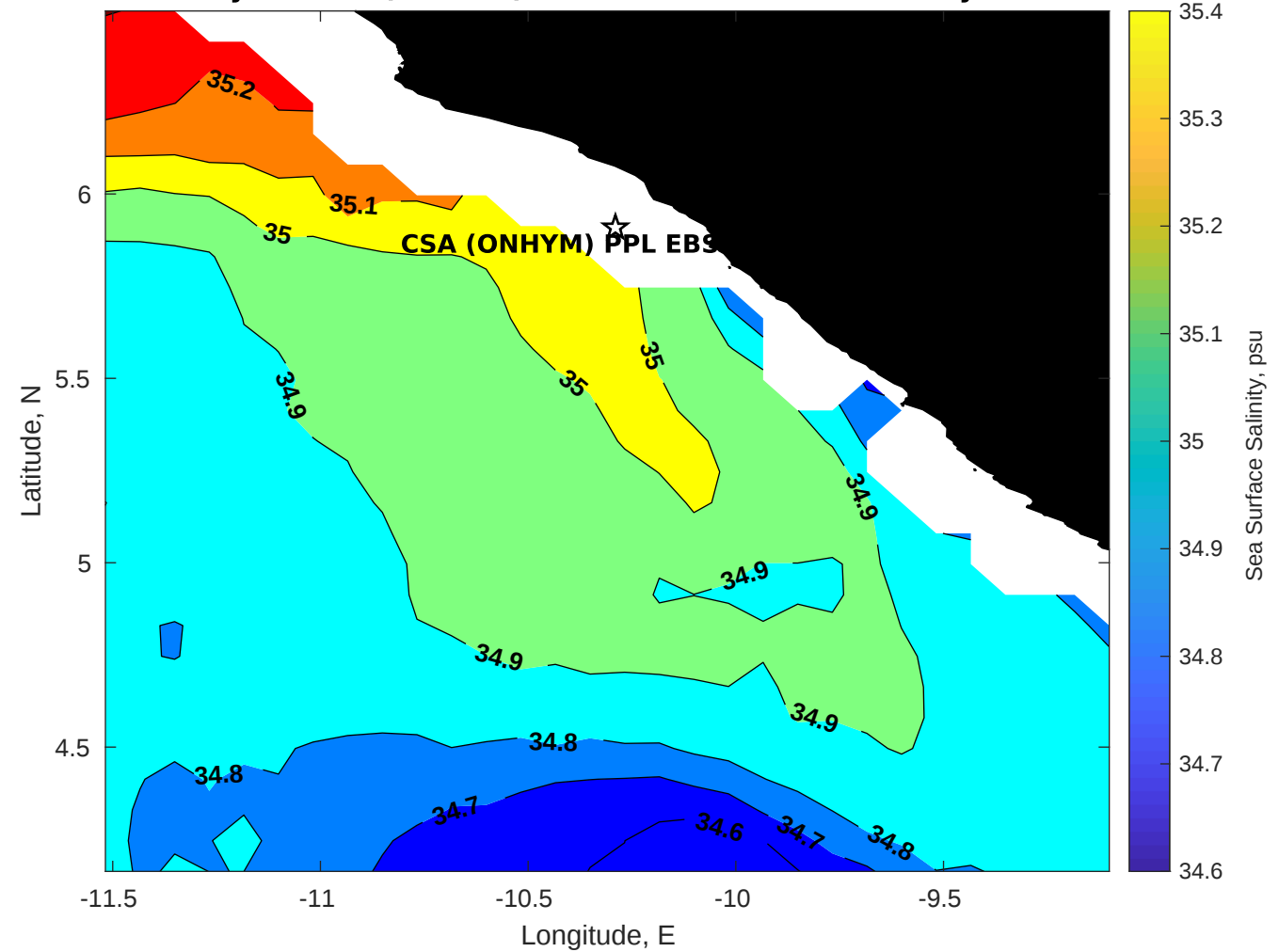
Surface Salinity for CSA (ONHYM) PPL EBS - Liberia at 07-May-2025 00:00:00
