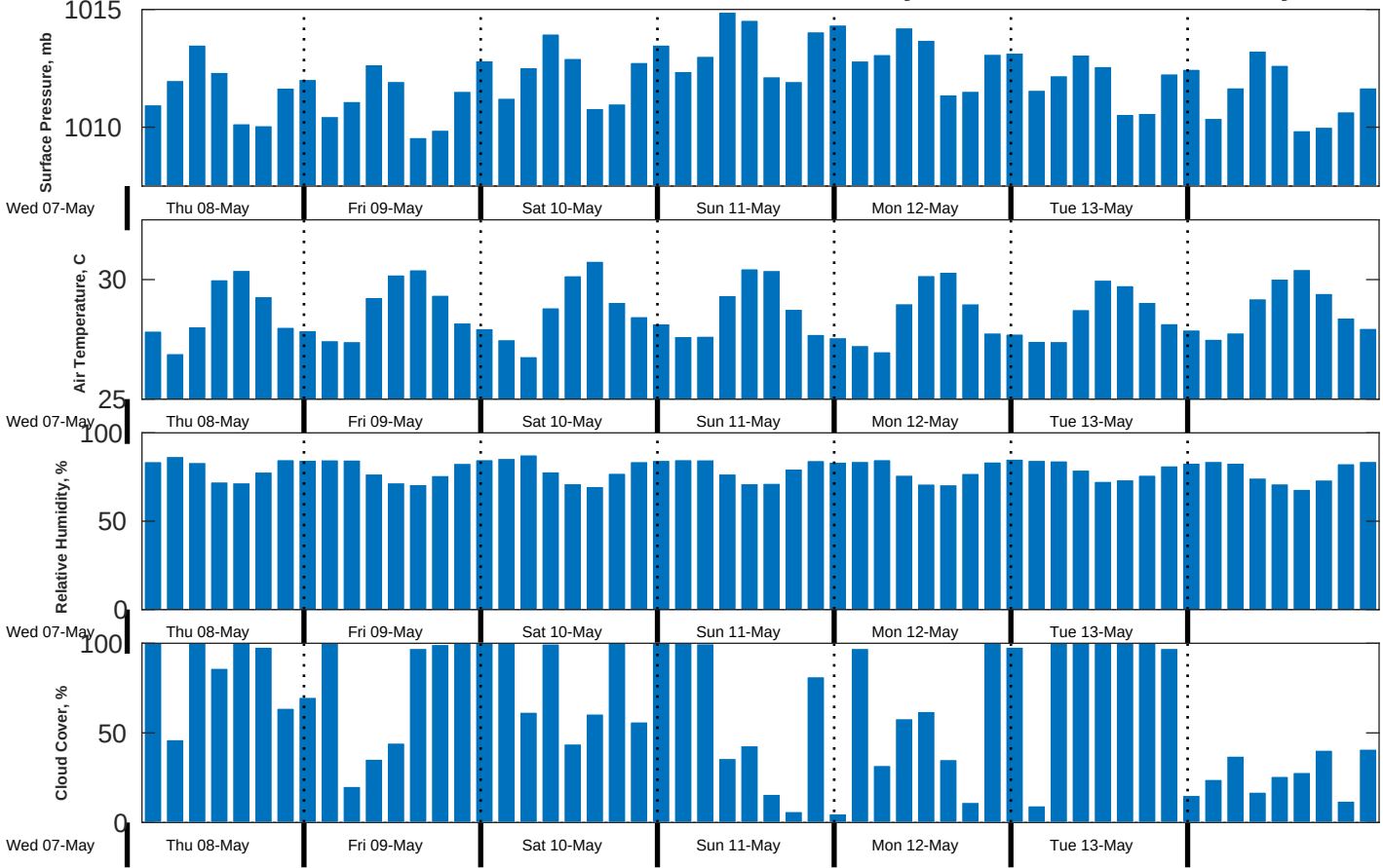
Met Forecast for CSA (ONHYM) PPL EBS - Liberia from 08-May-2025 00:00:00 to 15-May-2025 00:00:00
