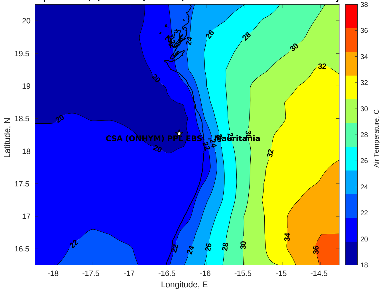
Air Temperature (C) for CSA (ONHYM) PPL EBS - Mauritania at 08-May-2025
