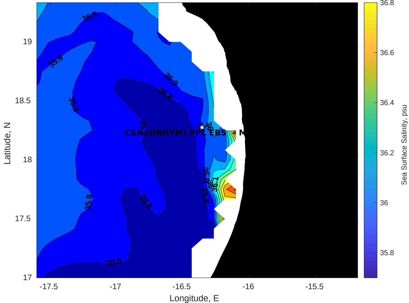
Surface Salinity for CSA (ONHYM) PPL EBS - Mauritania at 07-May-2025 00:00:00
