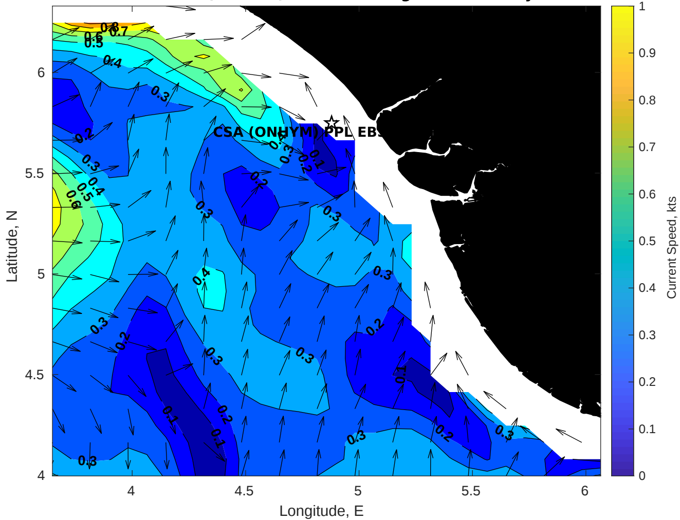
Surface Currents for CSA (ONHYM) PPL EBS - Nigeria at 07-May-2025 00:00:00
