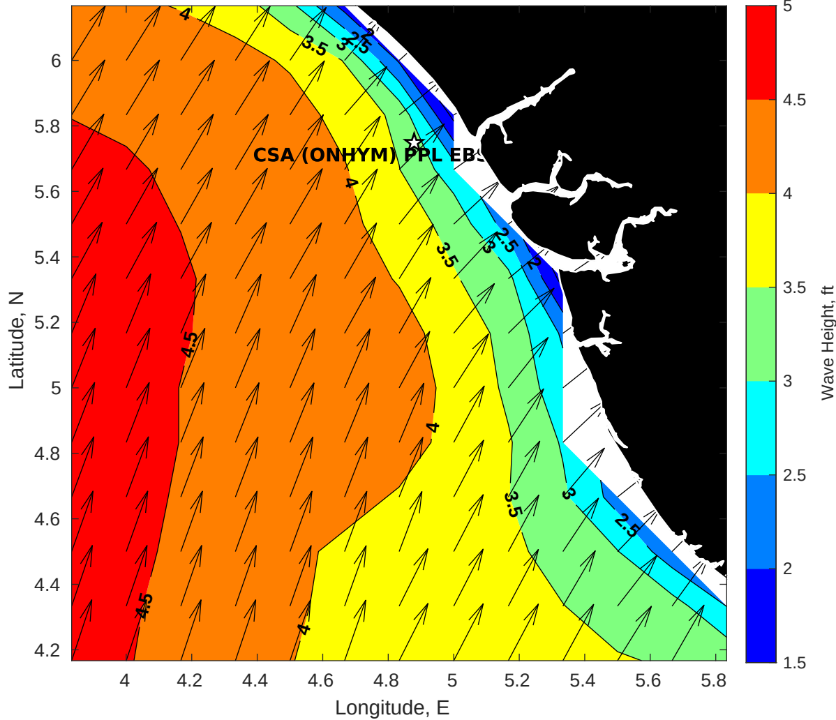
Wave Height (ft) for CSA (ONHYM) PPL EBS - Nigeria at 08-May-2025 09:00:00
