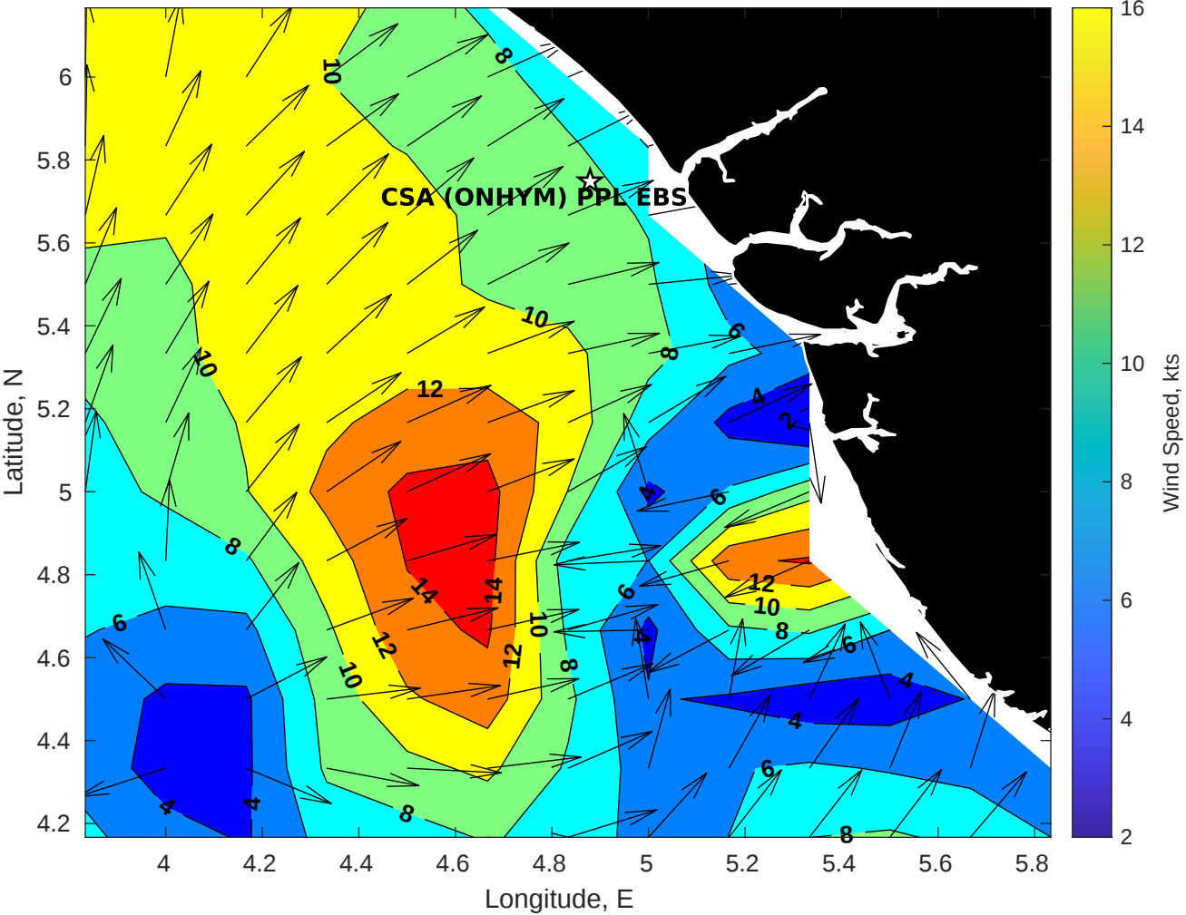
Winds (kts) for CSA (ONHYM) PPL EBS - Nigeria at 08-May-2025 09:00:00
