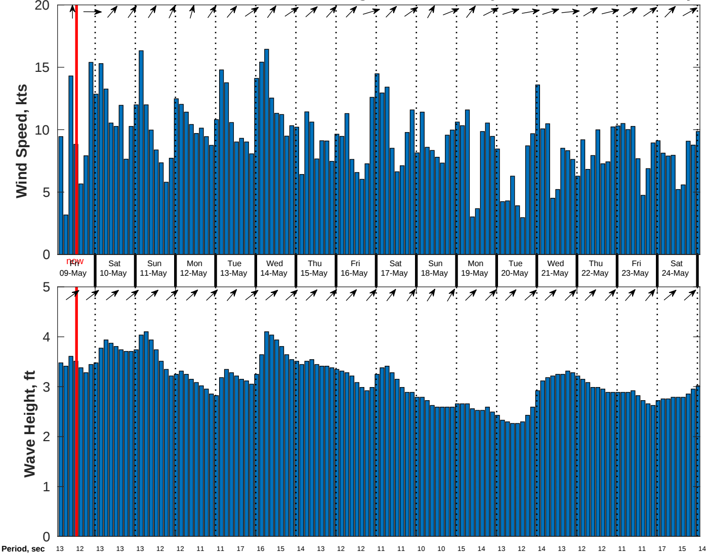
Wind & Wave Forecast for CSA (ONHYM) PPL EBS - Nigeria from 08-May-2025 02:00:00 to 24-May-2025 02:00:00
