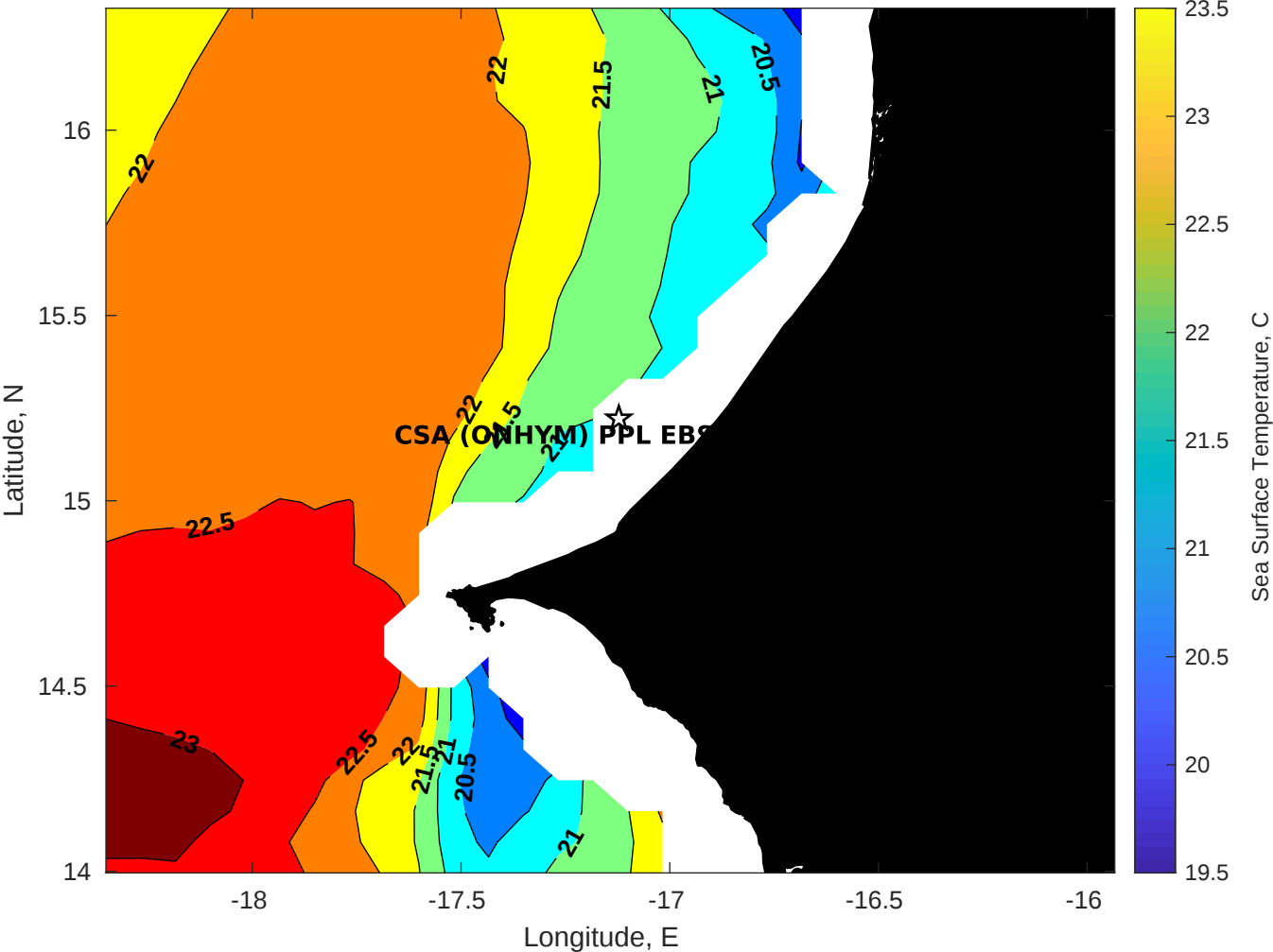
SST for CSA (ONHYM) PPL EBS - Senegal at 07-May-2025 00:00:00
