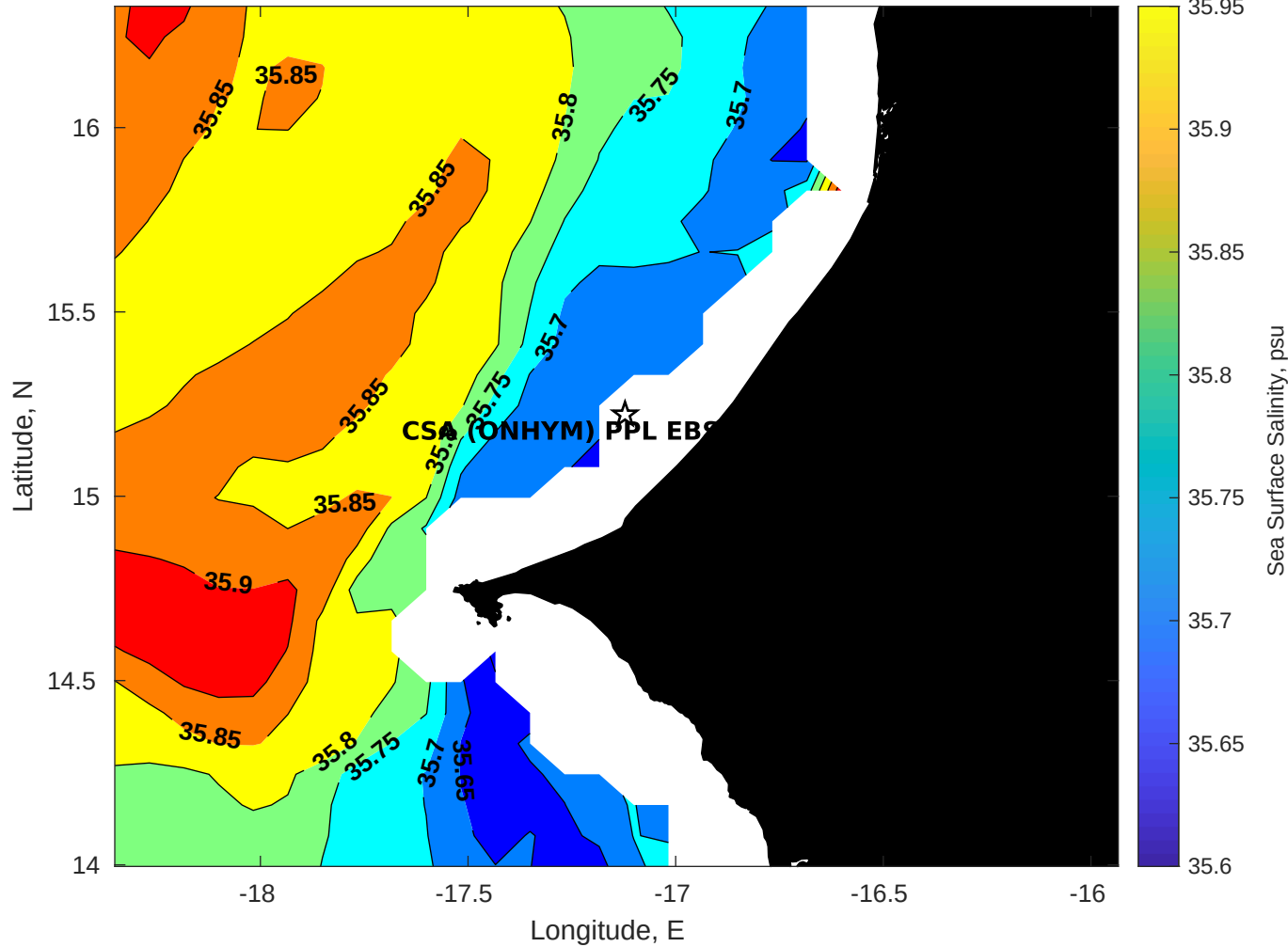
Surface Salinity for CSA (ONHYM) PPL EBS - Senegal at 07-May-2025 00:00:00
