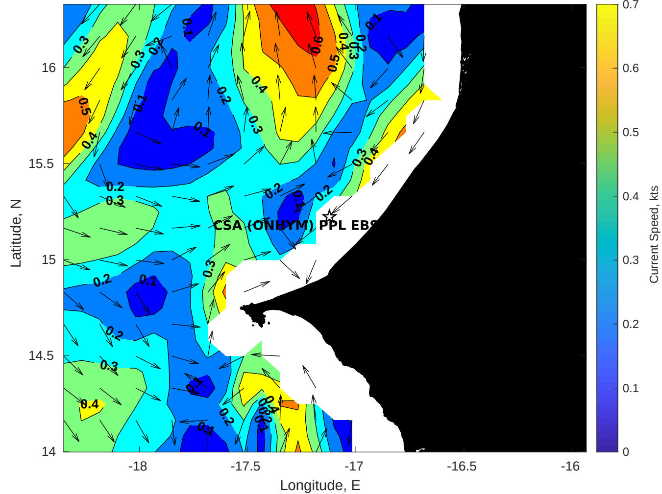
Surface Currents for CSA (ONHYM) PPL EBS - Senegal at 07-May-2025 00:00:00
