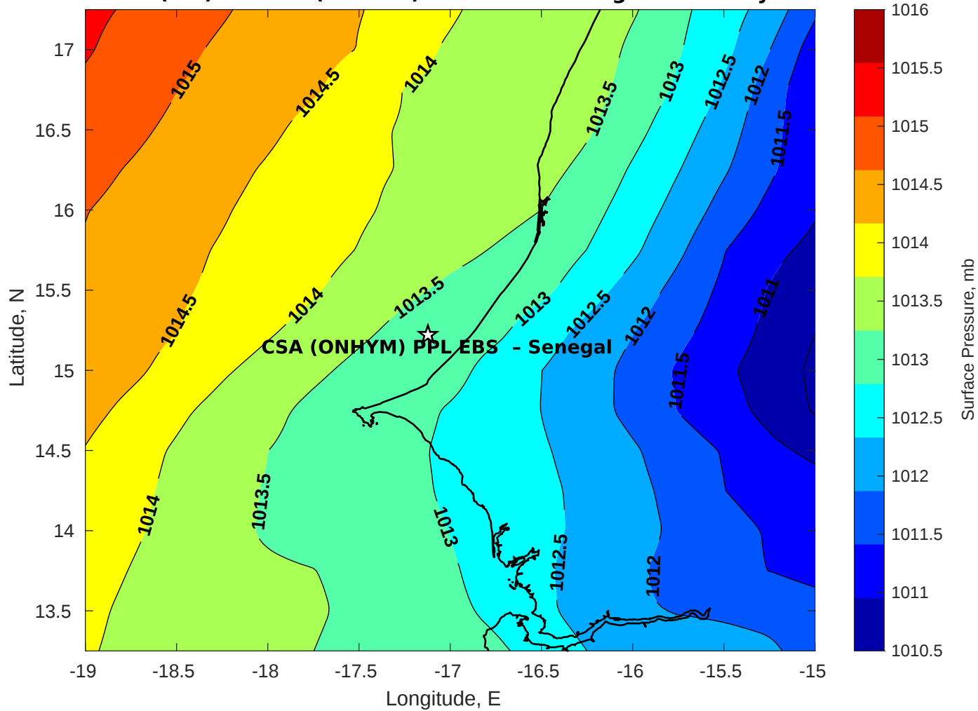
Surface Pressure (mb) for CSA (ONHYM) PPL EBS - Senegal at 10-May-2025 00:00:00
