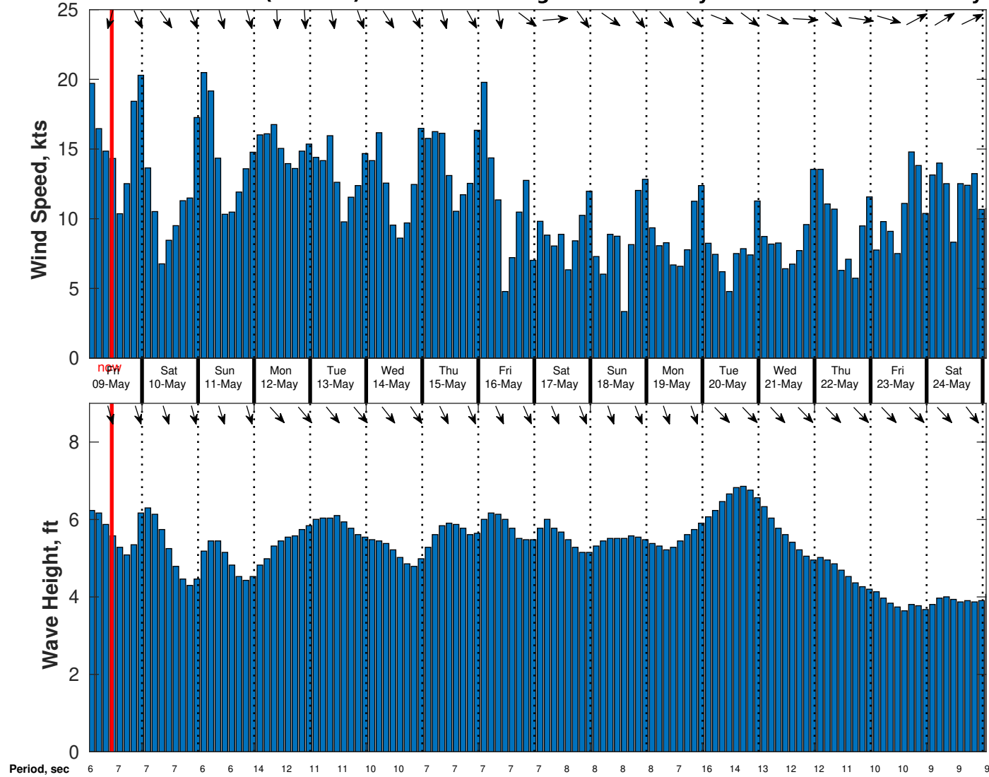
Wind & Wave Forecast for CSA (ONHYM) PPL EBS - Senegal from 08-May-2025 01:00:00 to 24-May-2025 01:00:00
