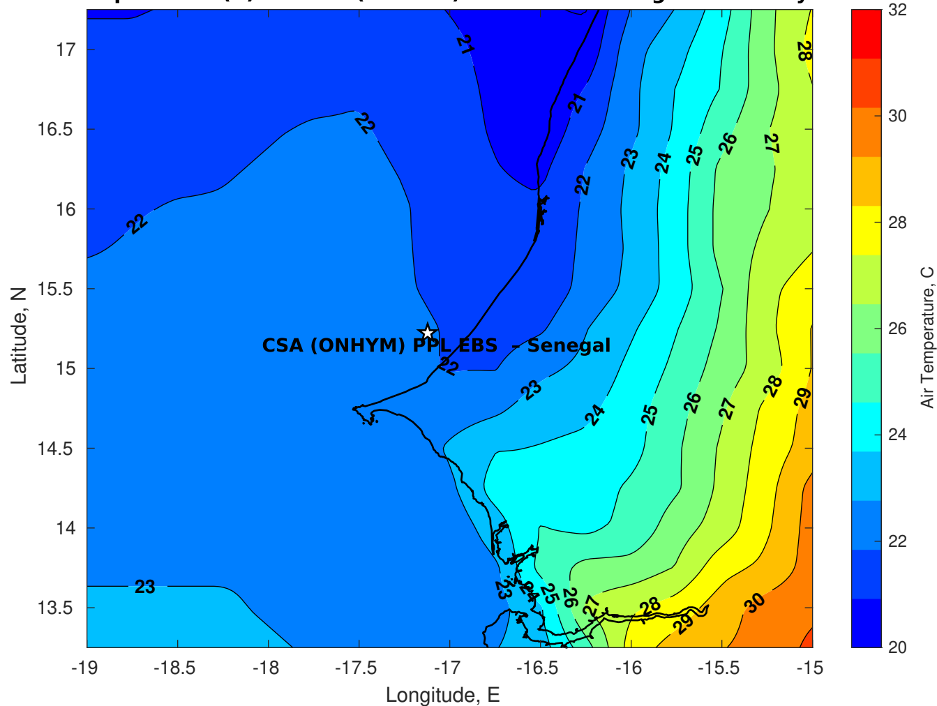
Air Temperature (C) for CSA (ONHYM) PPL EBS - Senegal at 08-May-2025
