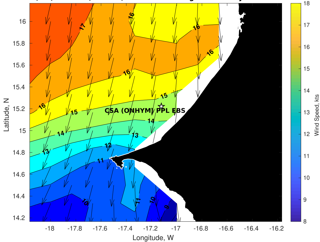
Winds (kts) for CSA (ONHYM) PPL EBS - Senegal at 08-May-2025 09:00:00
