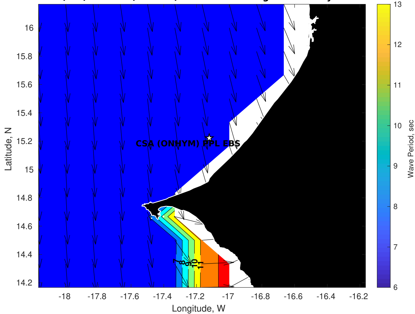
Wave Period (sec) for CSA (ONHYM) PPL EBS - Senegal at 08-May-2025 09:00:00
