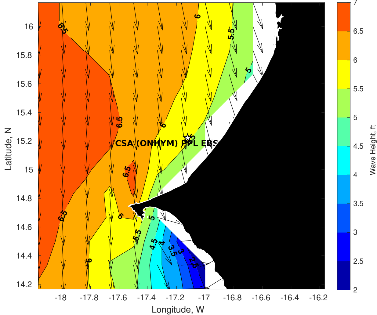
Wave Height (ft) for CSA (ONHYM) PPL EBS - Senegal at 08-May-2025 09:00:00
