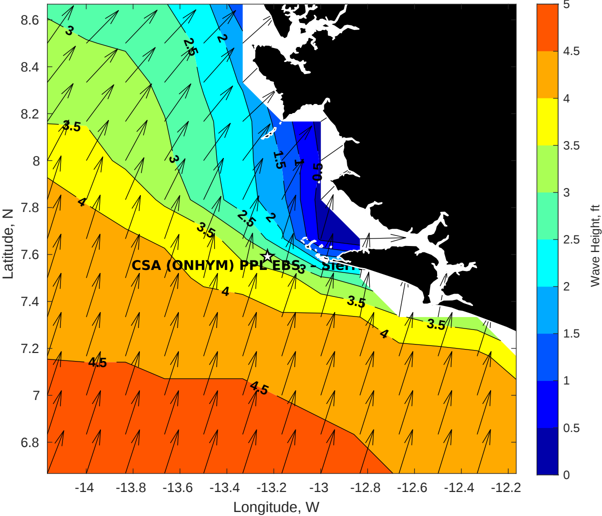
Wave Height (ft) for CSA (ONHYM) PPL EBS - Sierra Leone at 08-May-2025 09:00:00
