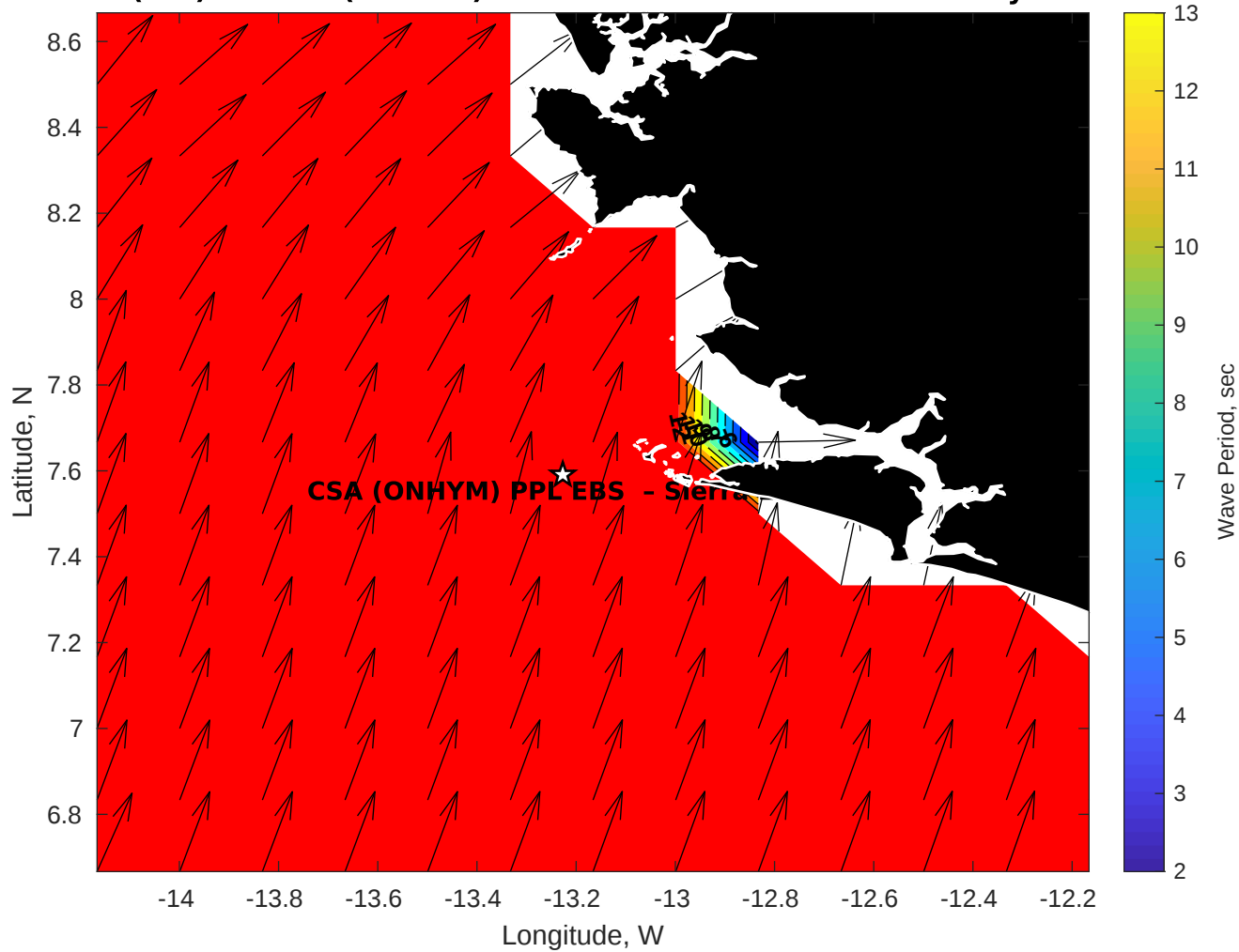
Wave Period (sec) for CSA (ONHYM) PPL EBS - Sierra Leone at 08-May-2025 09:00:00
