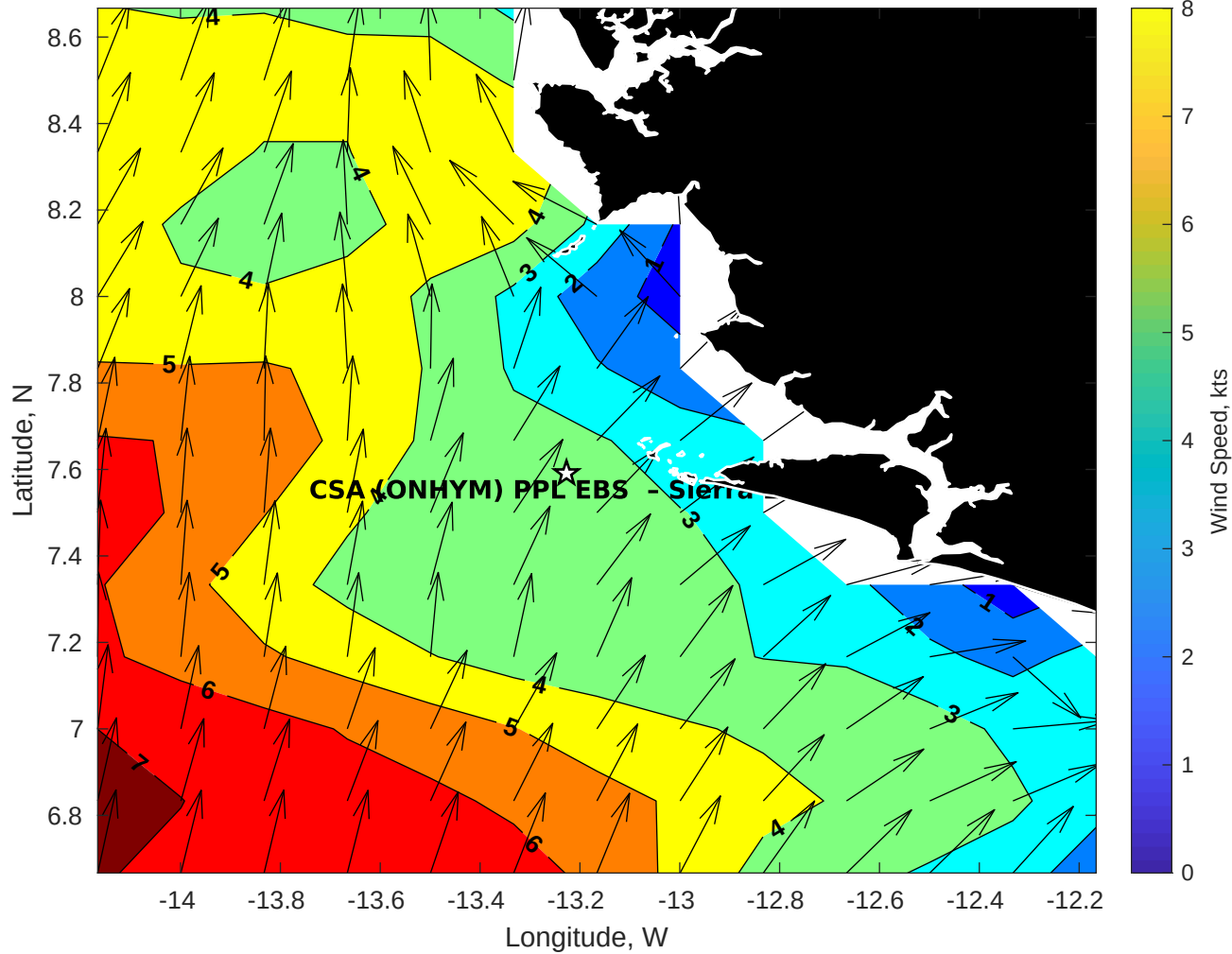
Winds (kts) for CSA (ONHYM) PPL EBS - Sierra Leone at 08-May-2025 09:00:00
