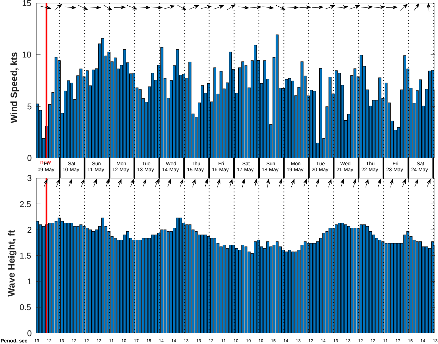
Wind & Wave Forecast for CSA (ONHYM) PPL EBS - Sierra Leone from 08-May-2025 01:00:00 to 24-May-2025 01:00:00
