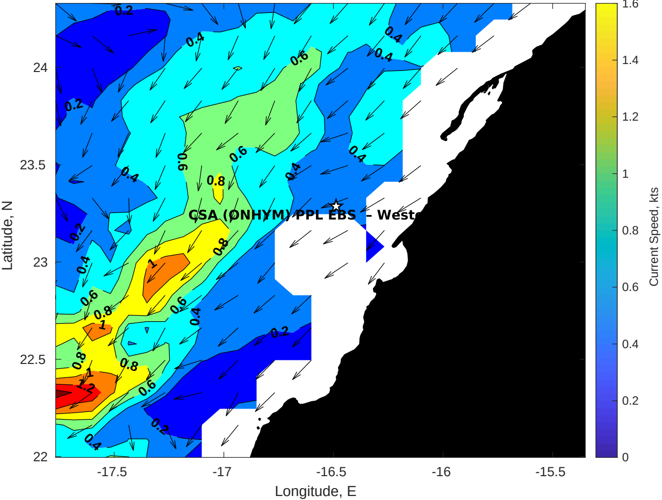
Surface Currents for CSA (ONHYM) PPL EBS - Western Sahara at 07-May-2025 00:00:00
