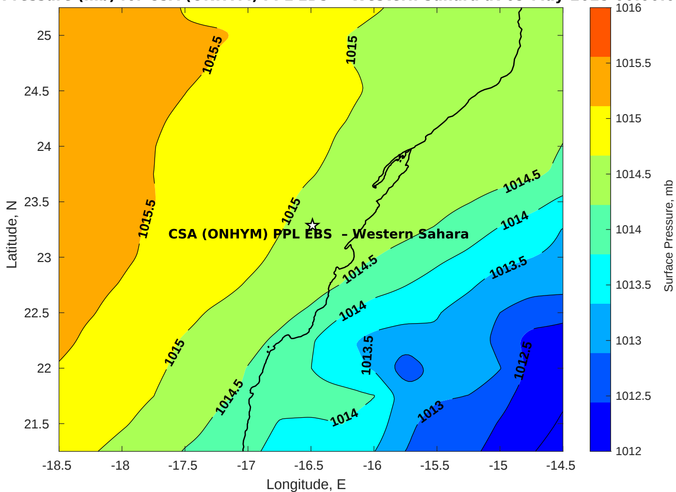
Surface Pressure (mb) for CSA (ONHYM) PPL EBS - Western Sahara at 09-May-2025 00:00:00
