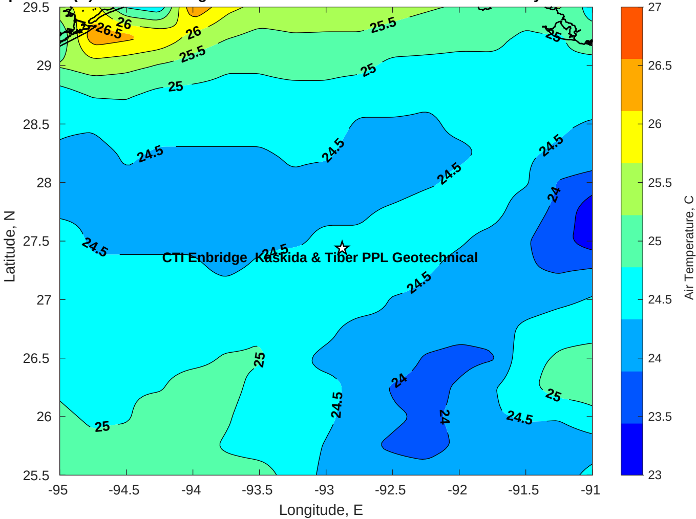
Air Temperature (C) for CTI Enbridge Kaskida & Tiber PPL Geotechnical at 08-May-2025
