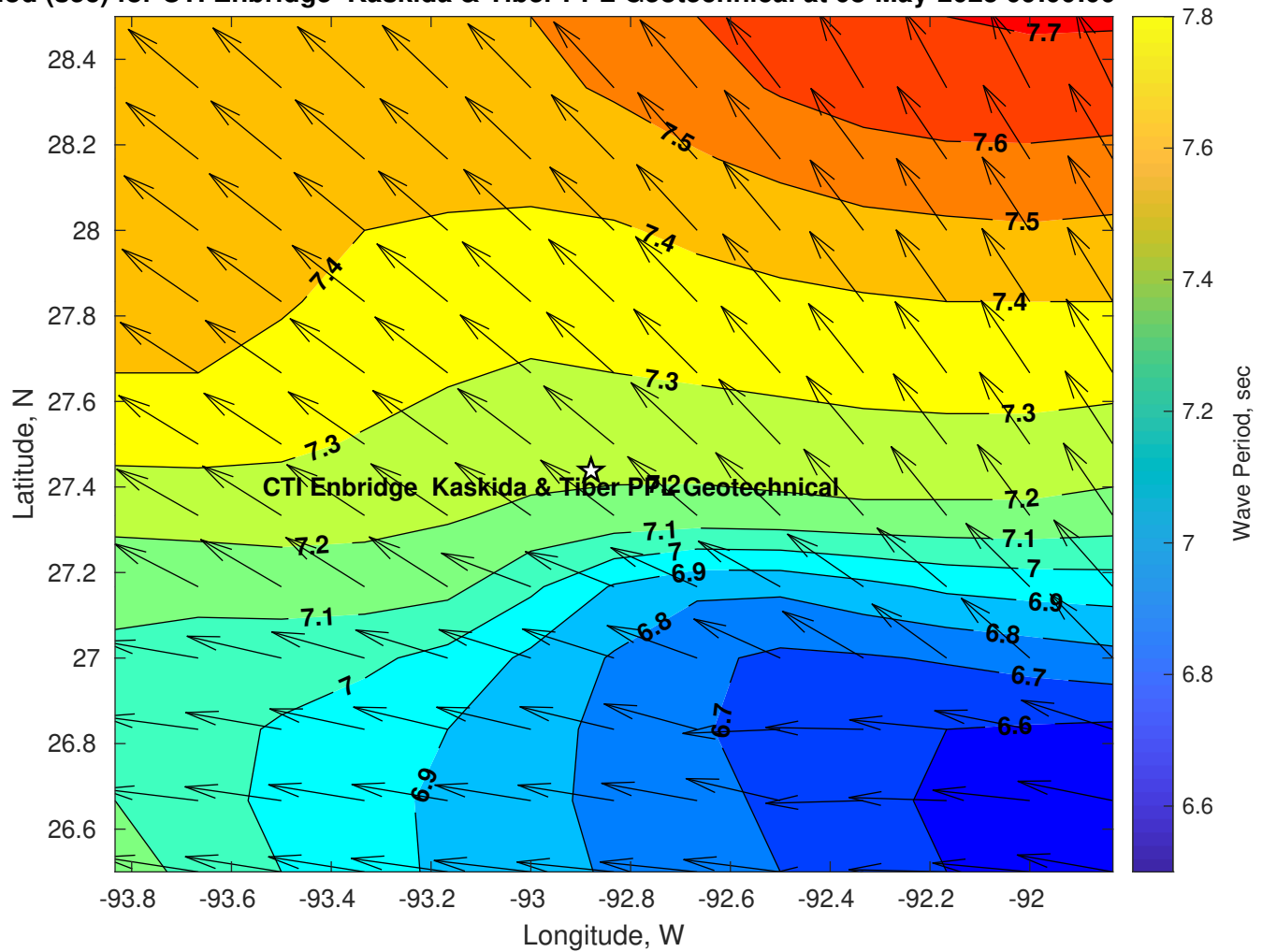
Wave Period (sec) for CTI Enbridge Kaskida & Tiber PPL Geotechnical at 08-May-2025 09:00:00
