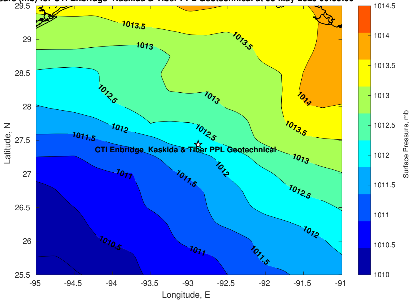
Surface Pressure (mb) for CTI Enbridge Kaskida & Tiber PPL Geotechnical at 08-May-2025 00:00:00
