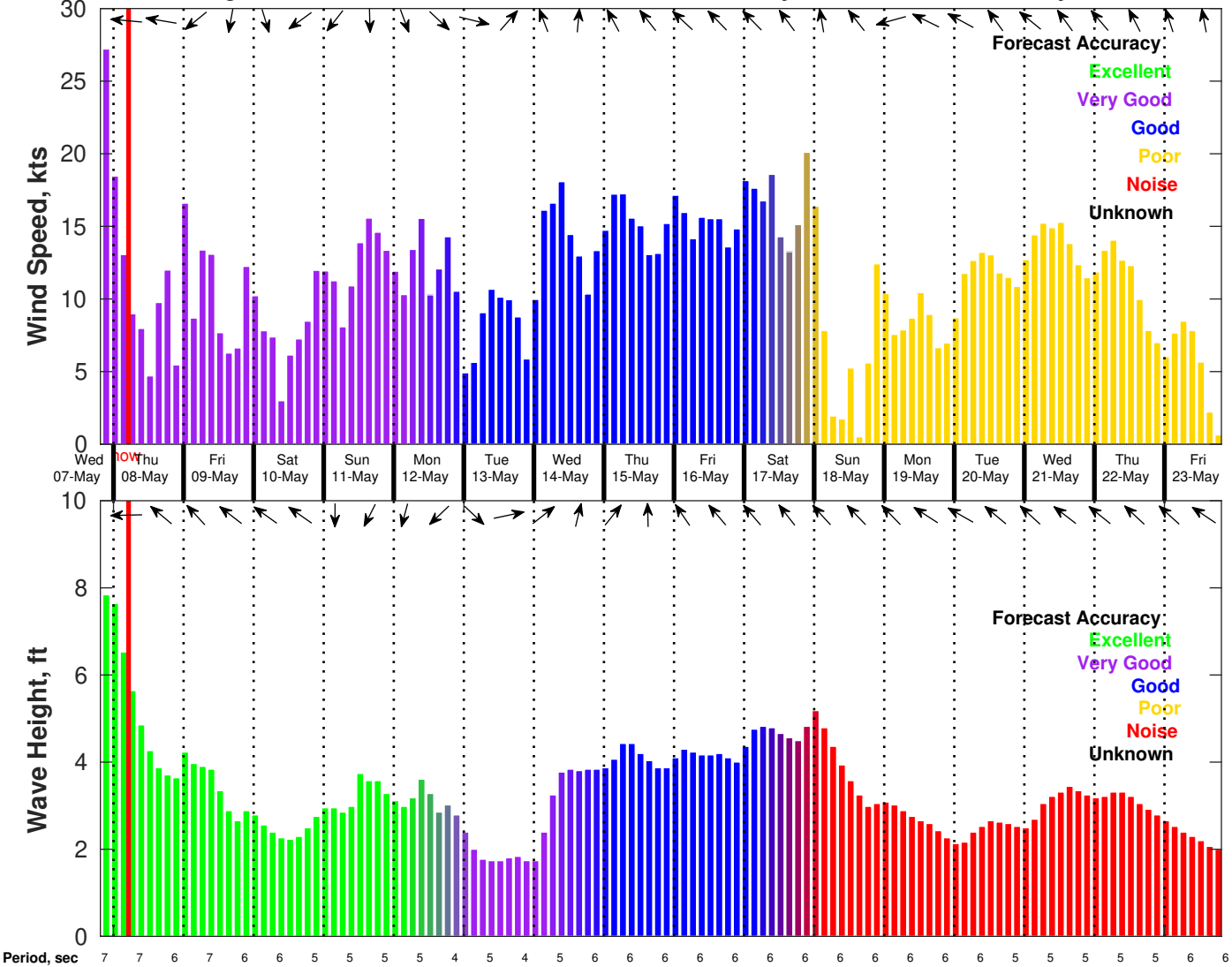
Wind & Wave Forecast for CTI Enbridge Kaskida & Tiber PPL Geotechnical from 07-May-2025 20:00:00 to 23-May-2025 20:00:00
