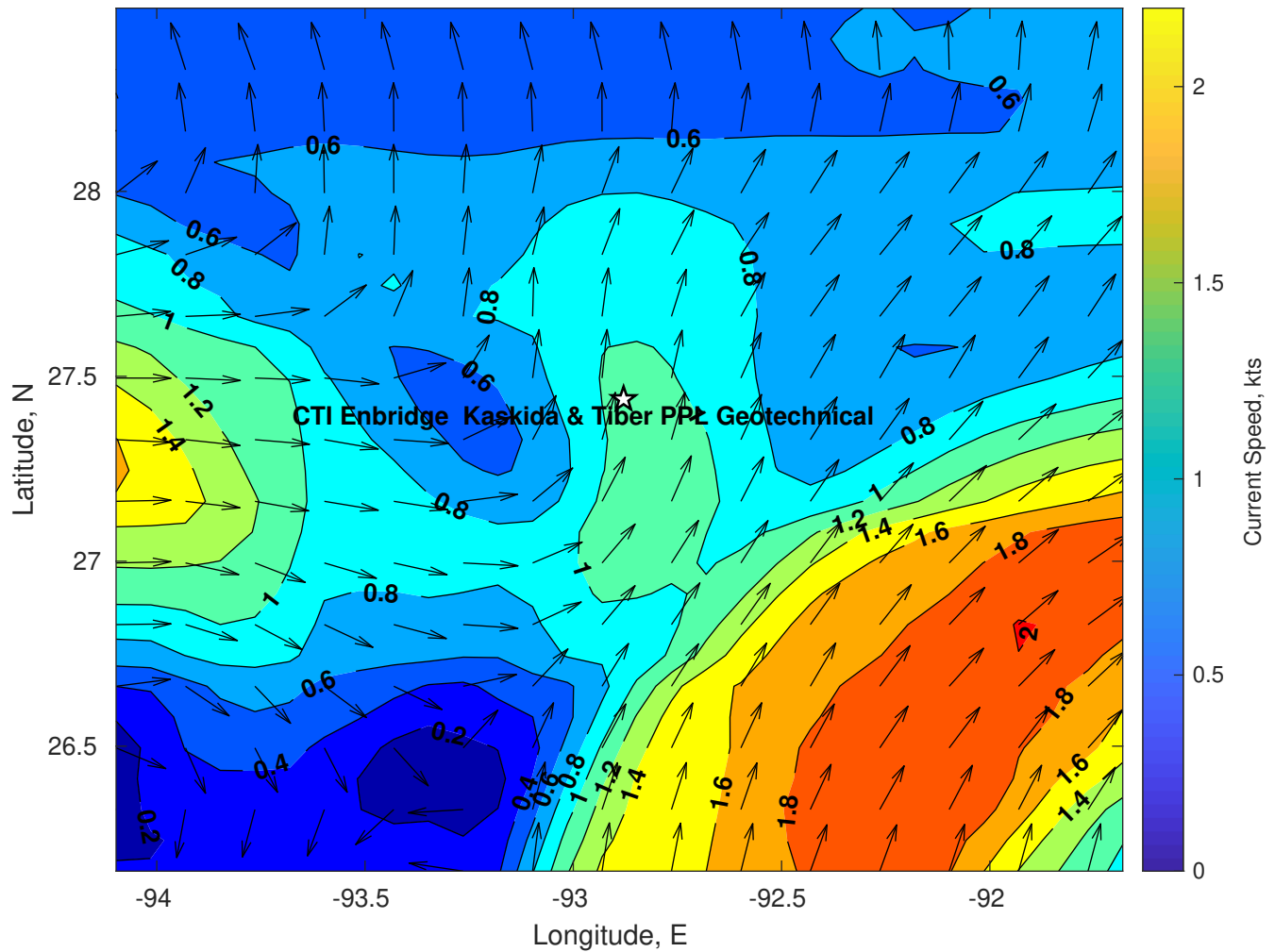
Surface Currents for CTI Enbridge Kaskida & Tiber PPL Geotechnical at 07-May-2025 00:00:00
