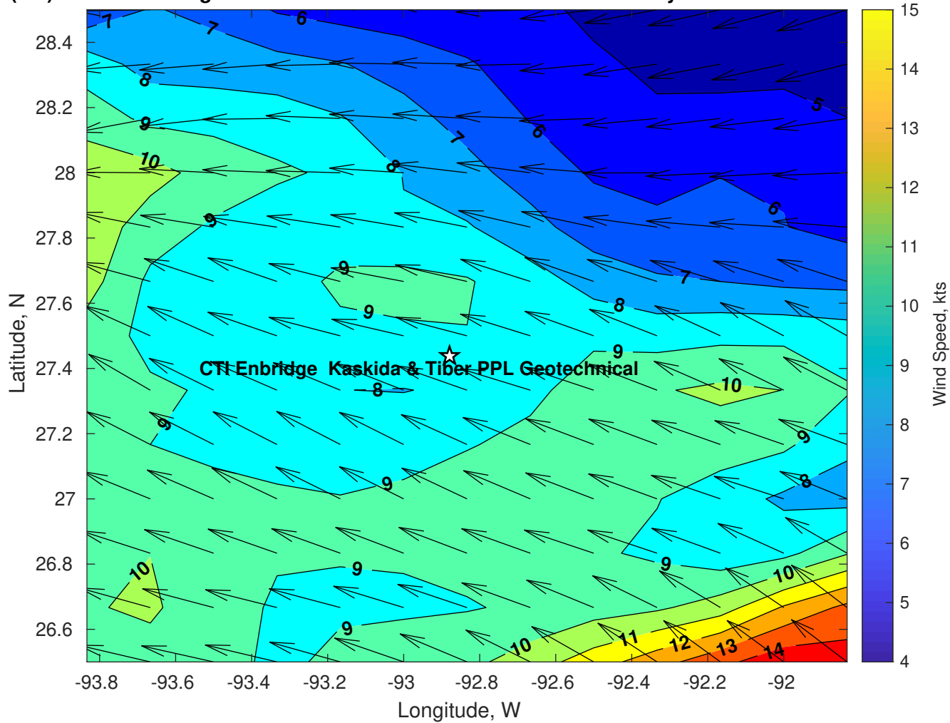
Winds (kts) for CTI Enbridge Kaskida & Tiber PPL Geotechnical at 08-May-2025 09:00:00
