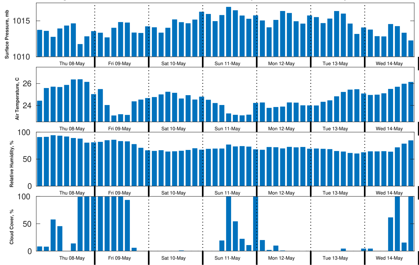
Met Forecast for CTI Enbridge Kaskida & Tiber PPL Geotechnical from 08-May-2025 00:00:00 to 15-May-2025 00:00:00
