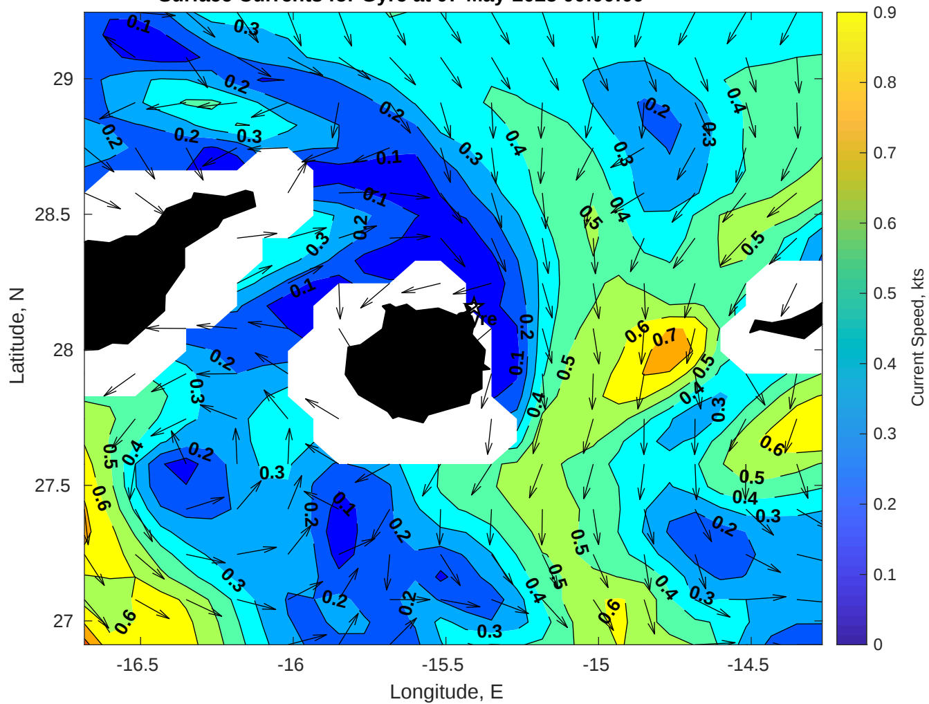
Surface Currents for Gyre at 07-May-2025 00:00:00
