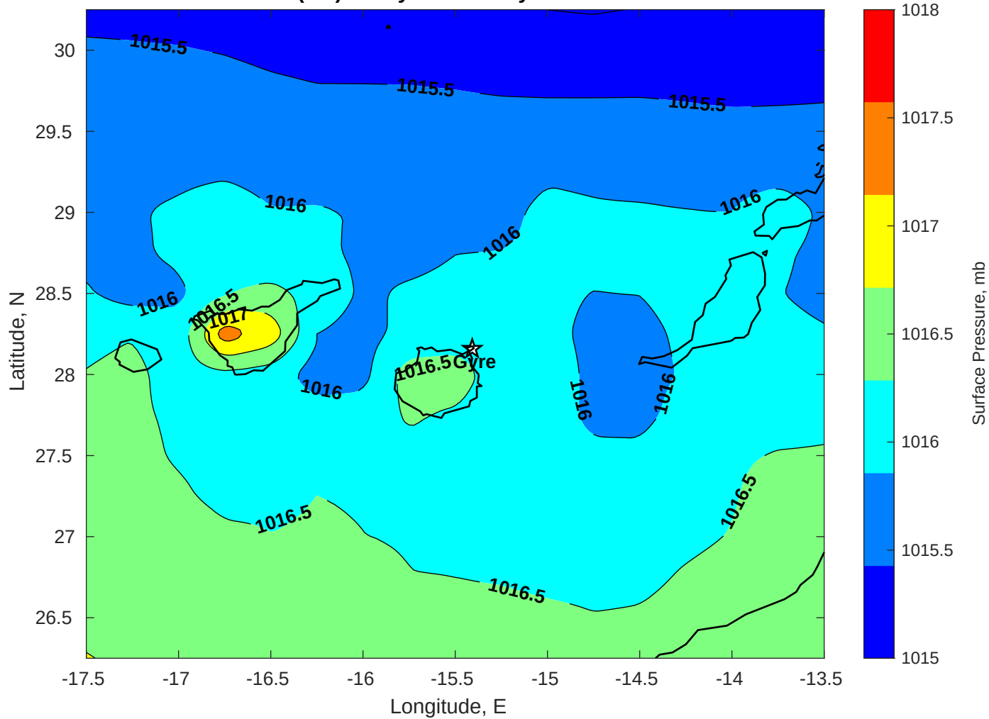
Surface Pressure (mb) for Gyre at 08-May-2025 00:00:00
