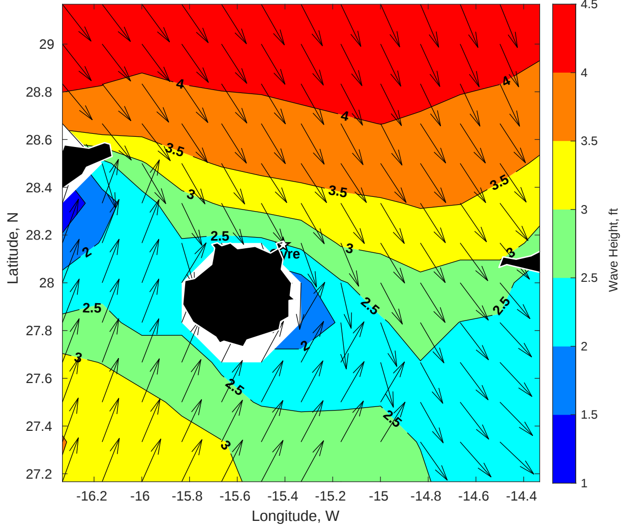
Wave Height (ft) for Gyre at 08-May-2025 09:00:00
