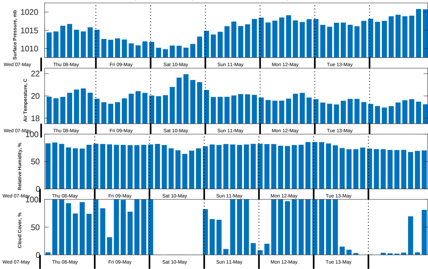
Met Forecast for Gyre from 07-May-2025 23:00:00 to 14-May-2025 23:00:00
