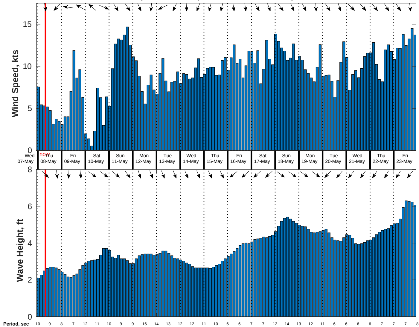
Wind & Wave Forecast for Gyre from 07-May-2025 23:00:00 to 23-May-2025 23:00:00
