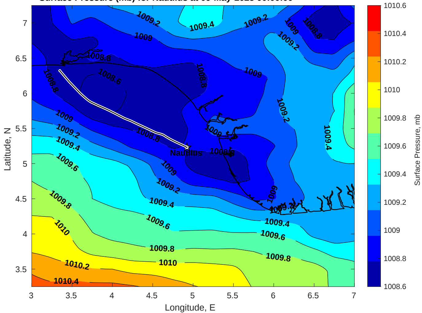
Surface Pressure (mb) for Nautilus at 09-May-2025 00:00:00
