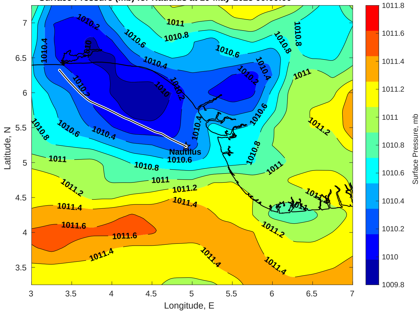
Surface Pressure (mb) for Nautilus at 10-May-2025 00:00:00
