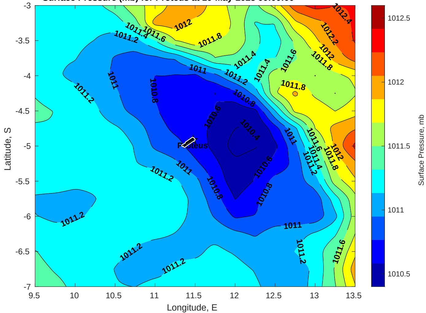
Surface Pressure (mb) for Proteus at 10-May-2025 00:00:00
