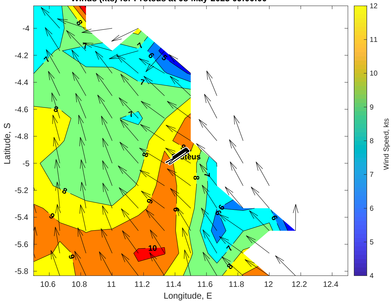
Winds (kts) for Proteus at 08-May-2025 09:00:00
