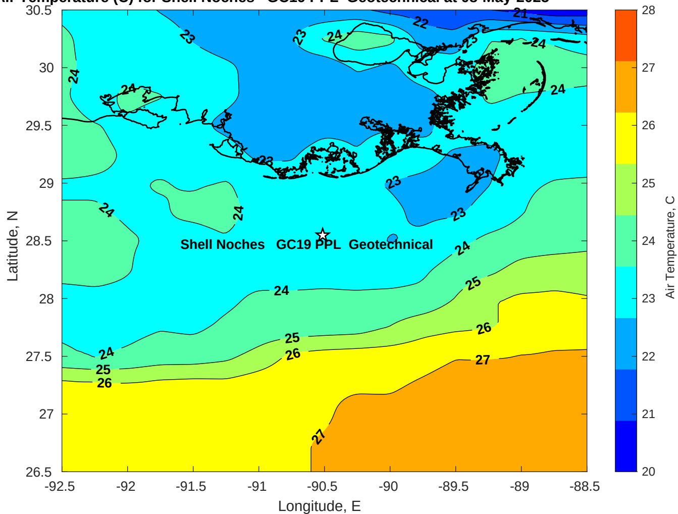
Air Temperature (C) for Shell Noches GC19 PPL Geotechnical at 08-May-2025
