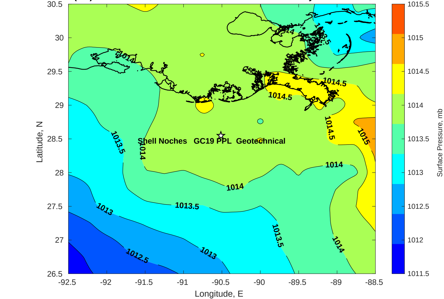
Surface Pressure (mb) for Shell Noches GC19 PPL Geotechnical at 08-May-2025 00:00:00
