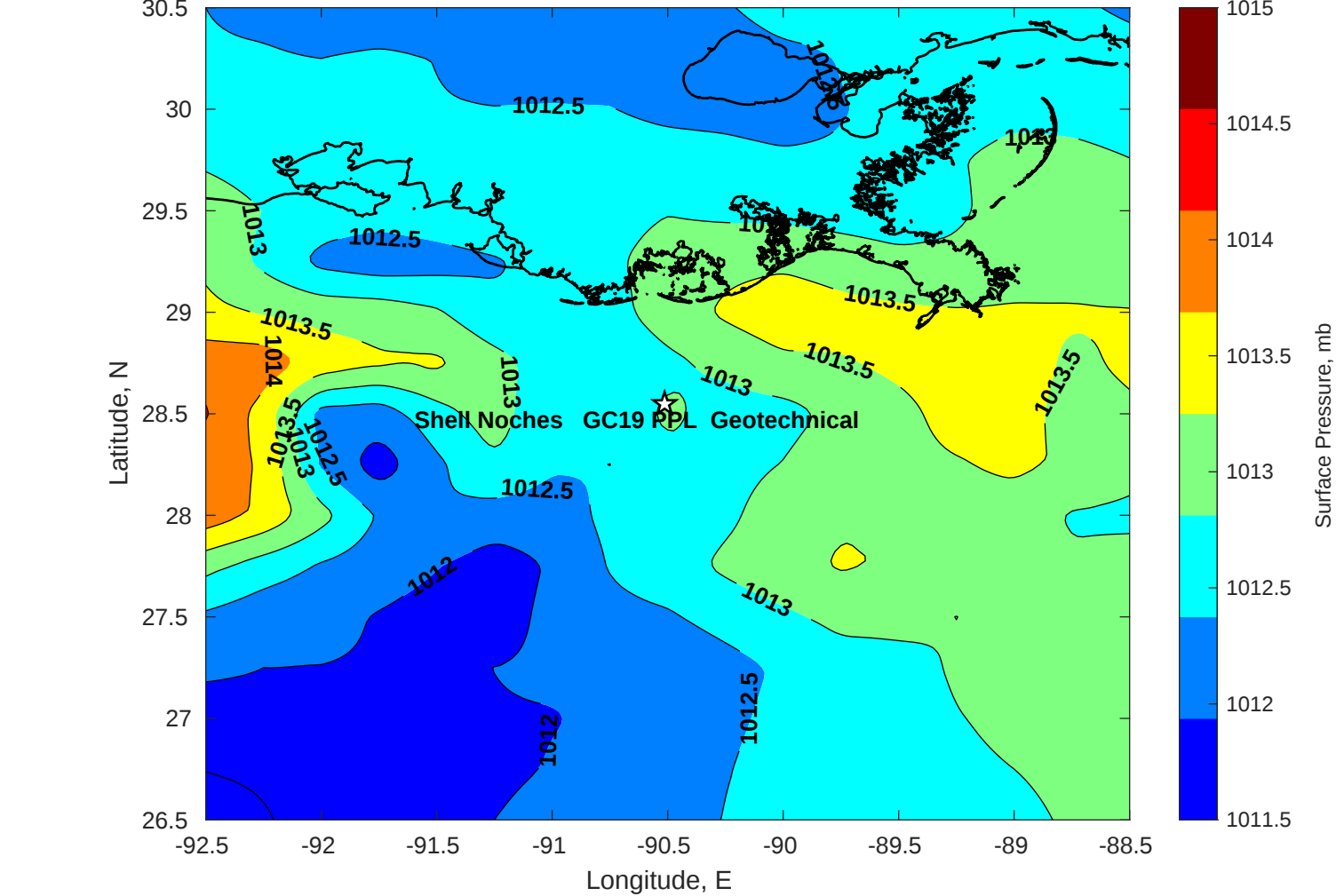
Surface Pressure (mb) for Shell Noches GC19 PPL Geotechnical at 09-May-2025 00:00:00
