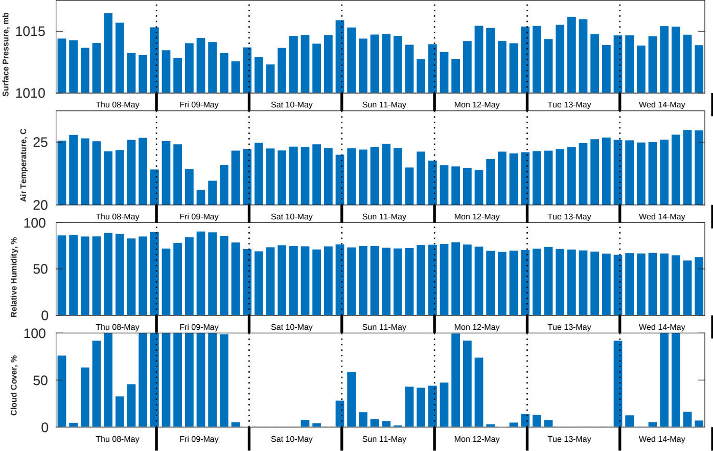
Met Forecast for Shell Noches GC19 PPL Geotechnical from 08-May-2025 00:00:00 to 15-May-2025 00:00:00
