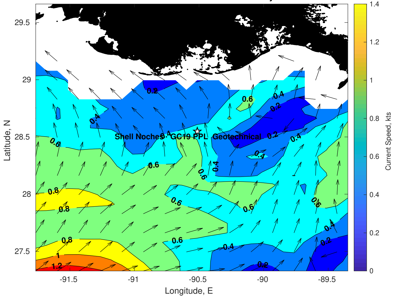
Surface Currents for Shell Noches GC19 PPL Geotechnical at 07-May-2025 00:00:00
