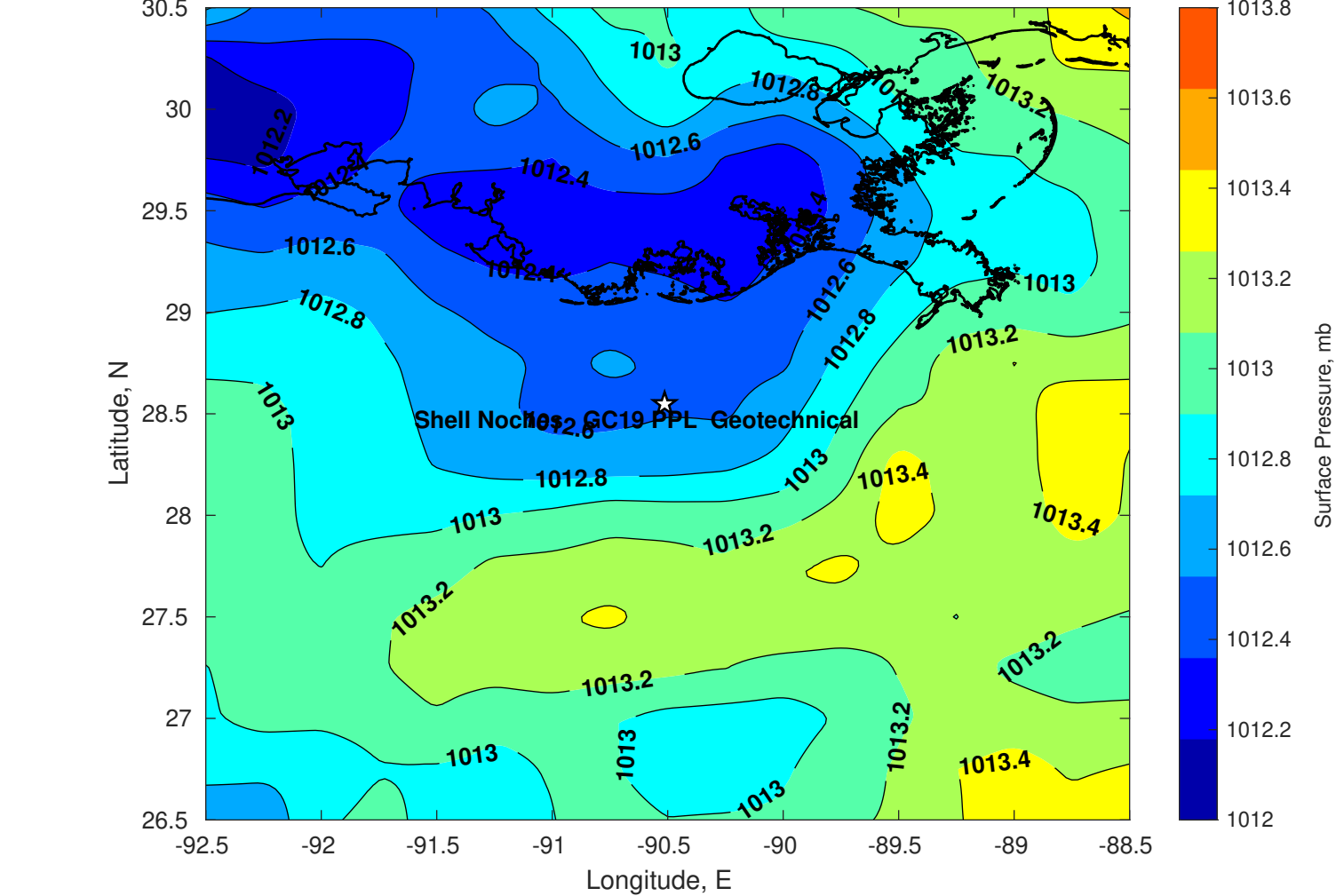
Surface Pressure (mb) for Shell Noches GC19 PPL Geotechnical at 10-May-2025 00:00:00
