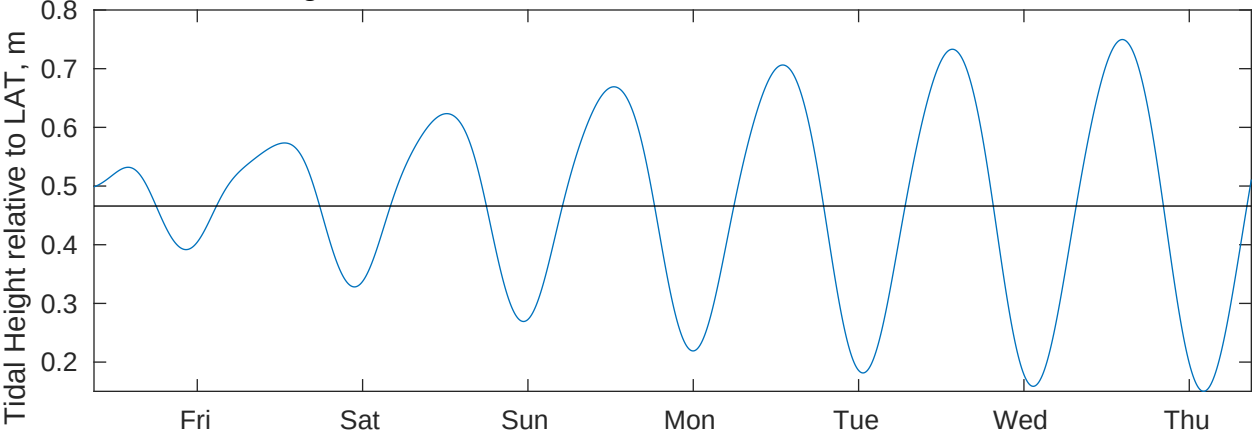
Tidal Currents and Heights for Shell Noches GC19 PPL Geotechnical at 20250508
