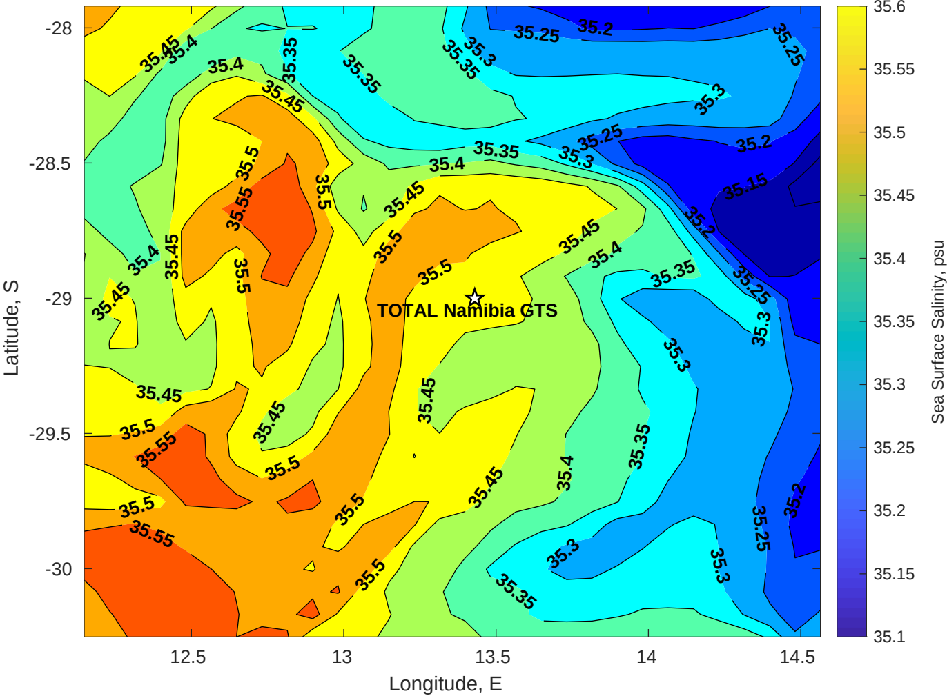
Surface Salinity for TOTAL Namibia GTS at 07-May-2025 00:00:00
