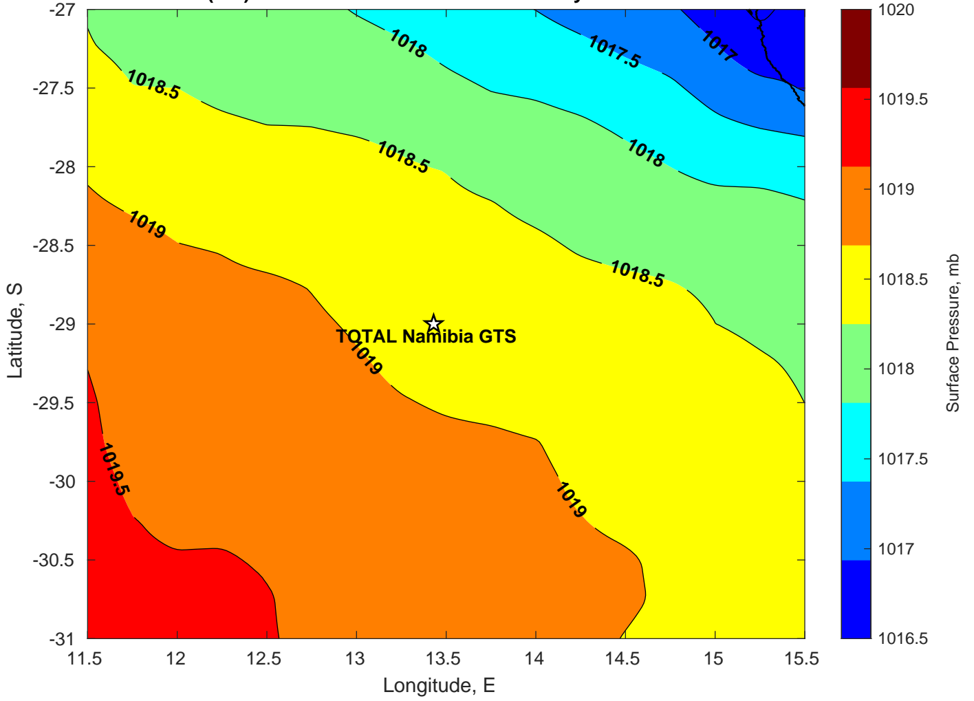
Surface Pressure (mb) for TOTAL Namibia GTS at 08-May-2025 00:00:00
