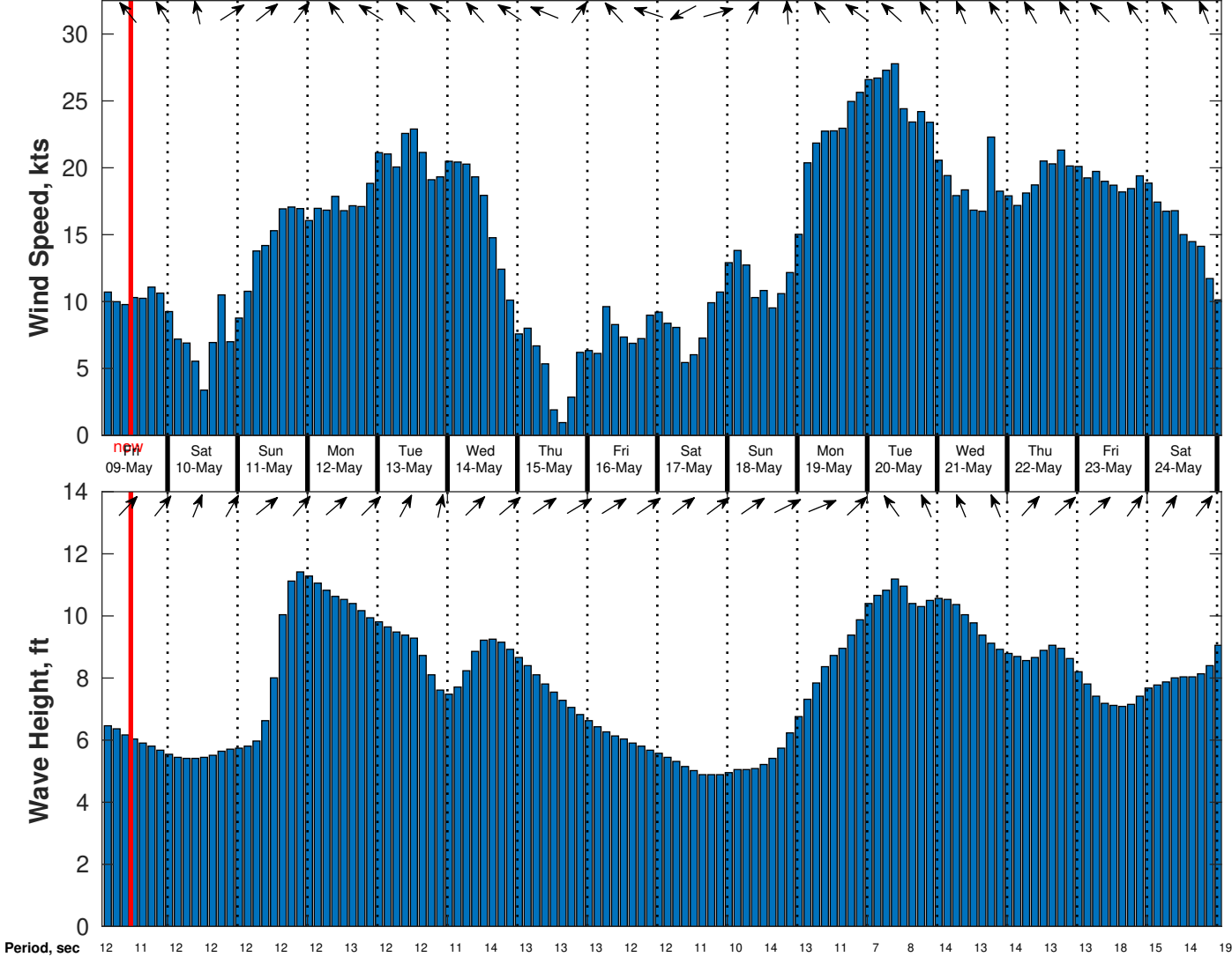
Wind & Wave Forecast for TOTAL Namibia GTS from 08-May-2025 02:00:00 to 24-May-2025 02:00:00
