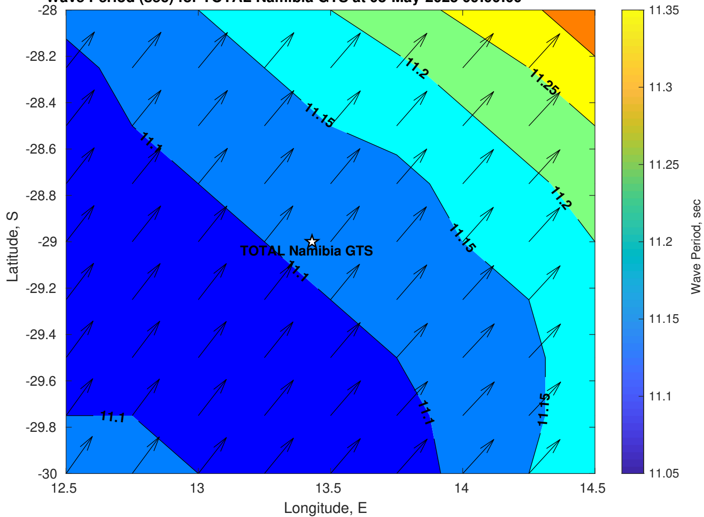
Wave Period (sec) for TOTAL Namibia GTS at 08-May-2025 09:00:00
