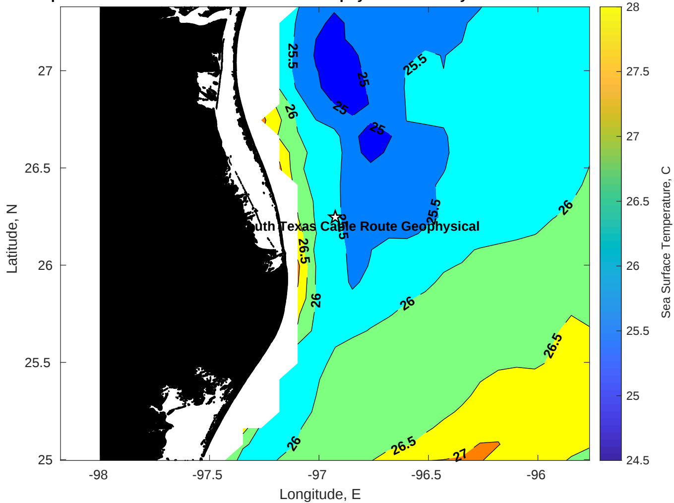
SST for Tampnet P2378 South Texas Cable Route Geophysical at 07-May-2025 00:00:00
