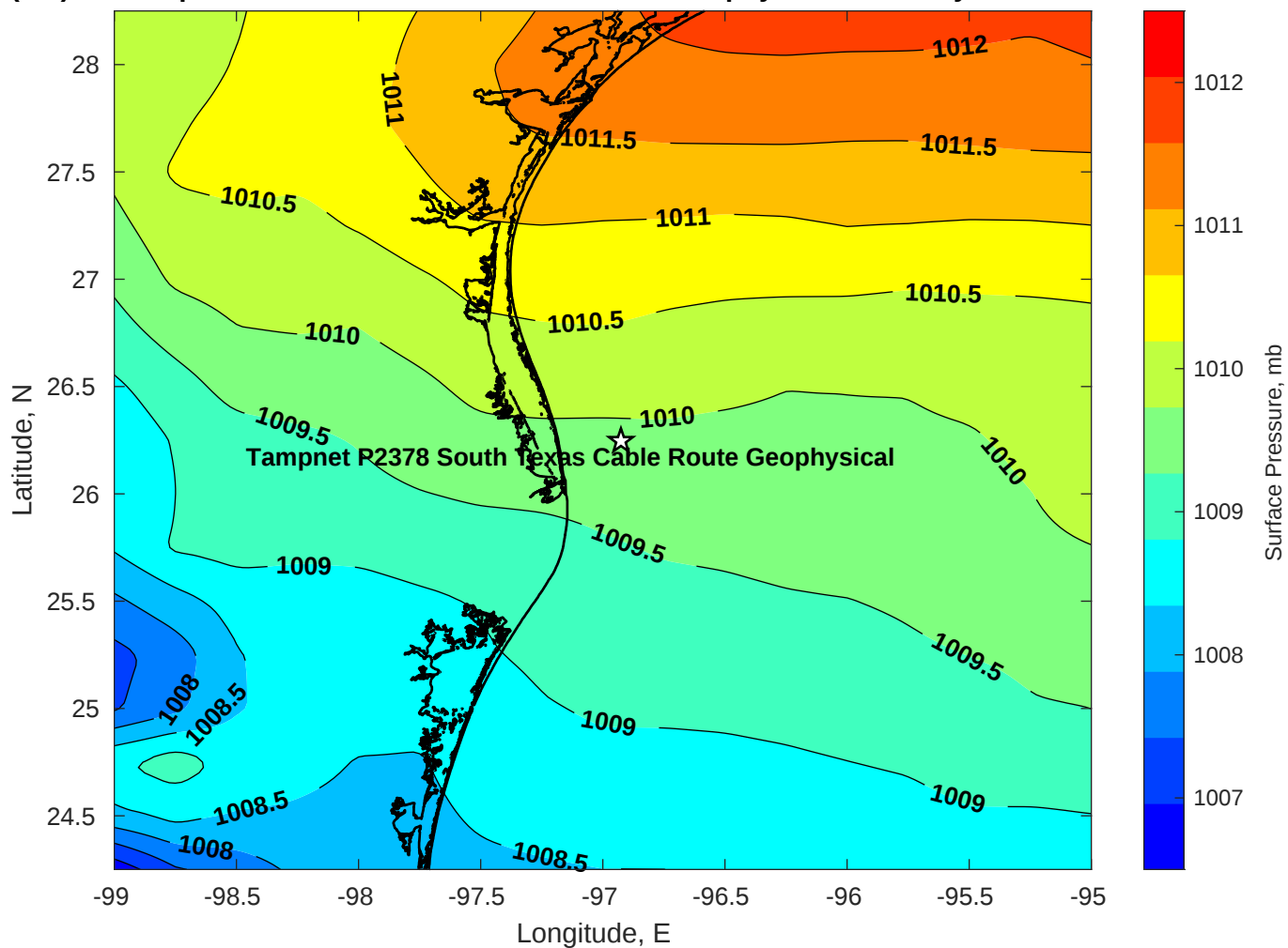
Pressure (mb) for Tampnet P2378 South Texas Cable Route Geophysical at 08-May-2025 00:00:00
