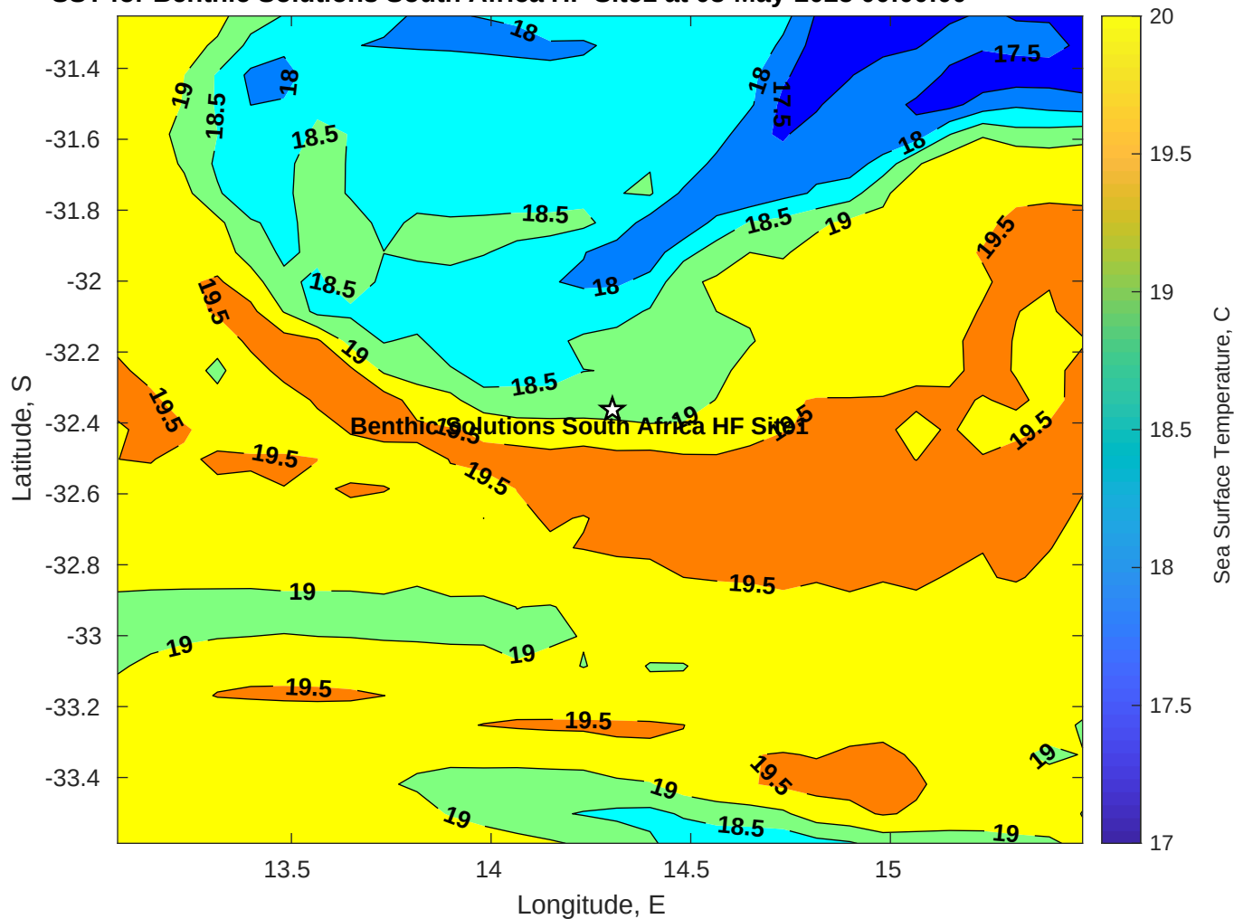
SST for Benthic Solutions South Africa HF Site1 at 08-May-2025 00:00:00
