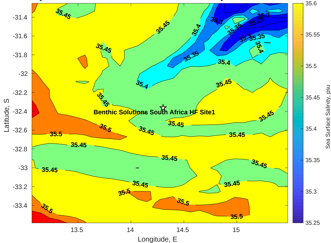
Surface Salinity for Benthic Solutions South Africa HF Site1 at 08-May-2025 00:00:00
