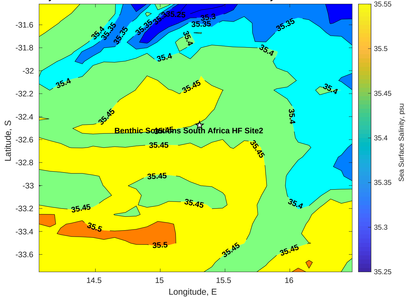
Surface Salinity for Benthic Solutions South Africa HF Site2 at 08-May-2025 00:00:00
