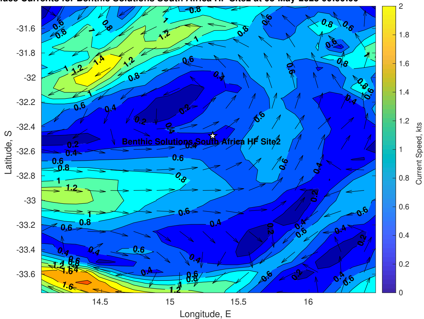
Surface Currents for Benthic Solutions South Africa HF Site2 at 08-May-2025 00:00:00
