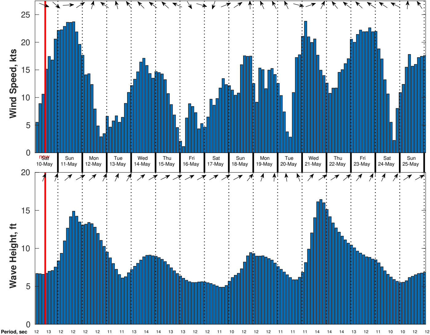
Wind & Wave Forecast for Benthic Solutions South Africa HF Site2 from 09-May-2025 02:00:00 to 25-May-2025 02:00:00
