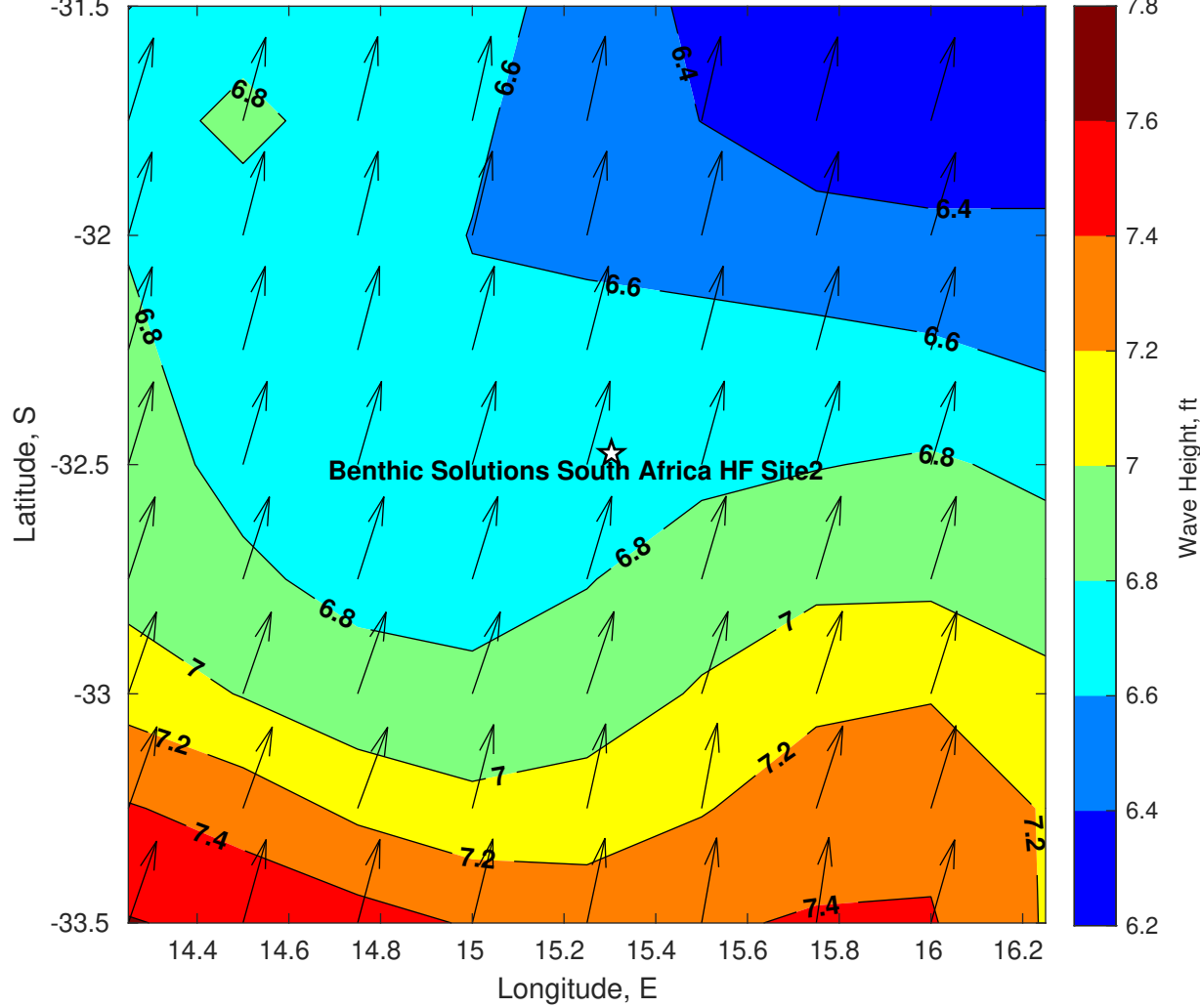
Wave Height (ft) for Benthic Solutions South Africa HF Site2 at 09-May-2025 09:00:00
