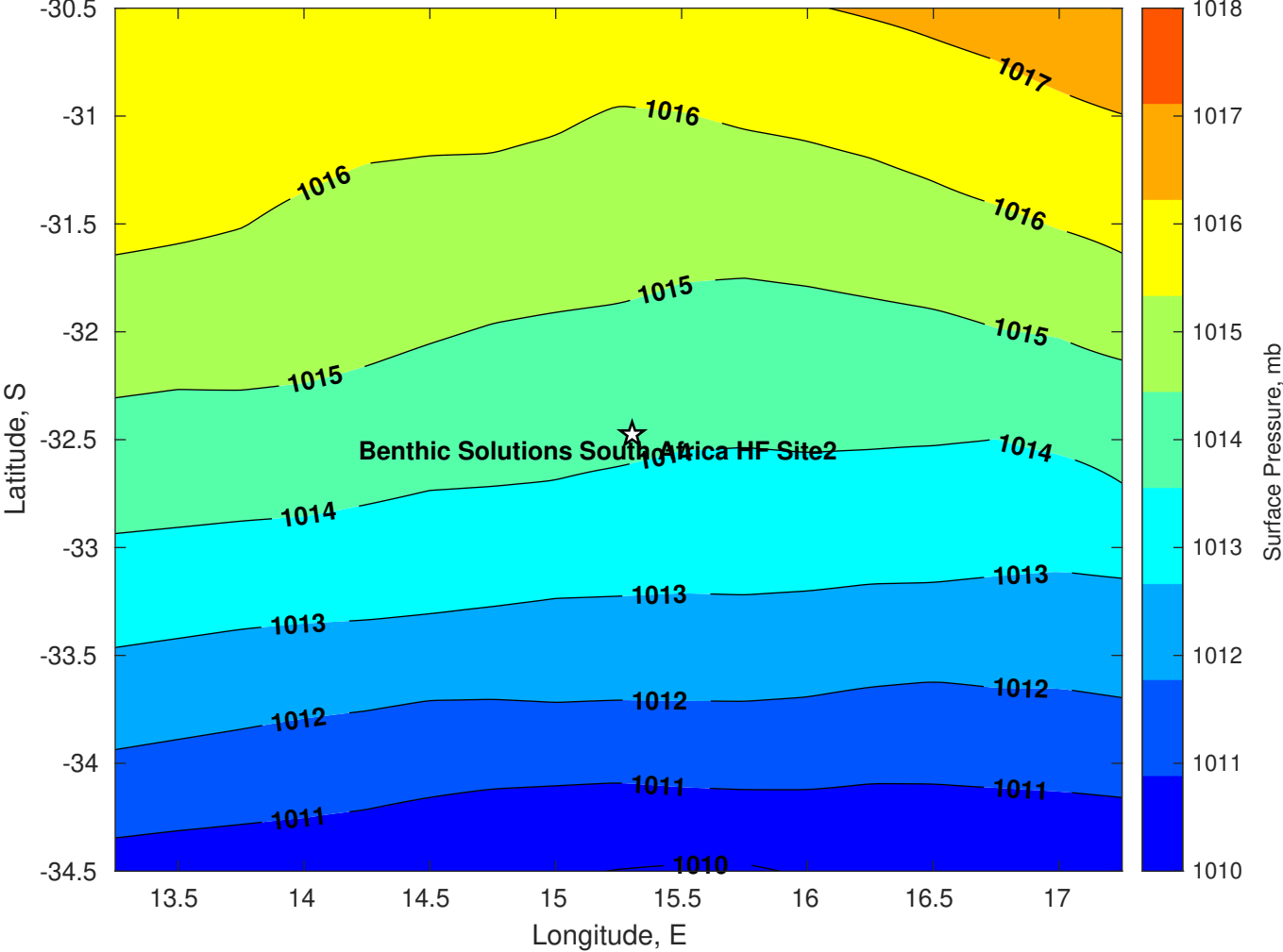
Surface Pressure (mb) for Benthic Solutions South Africa HF Site2 at 10-May-2025 00:00:00
