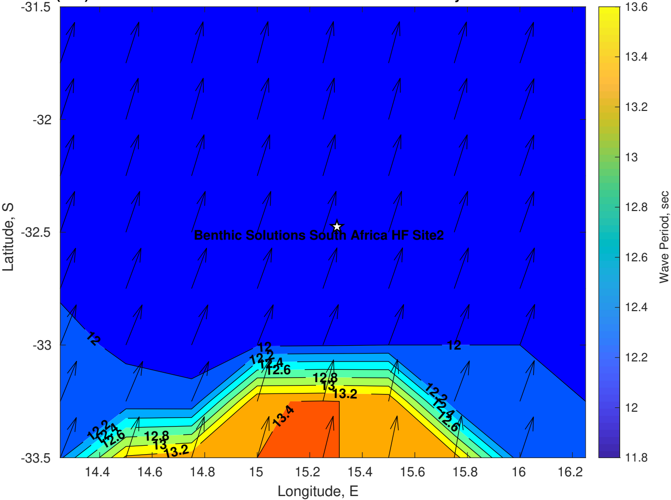
Wave Period (sec) for Benthic Solutions South Africa HF Site2 at 09-May-2025 09:00:00
