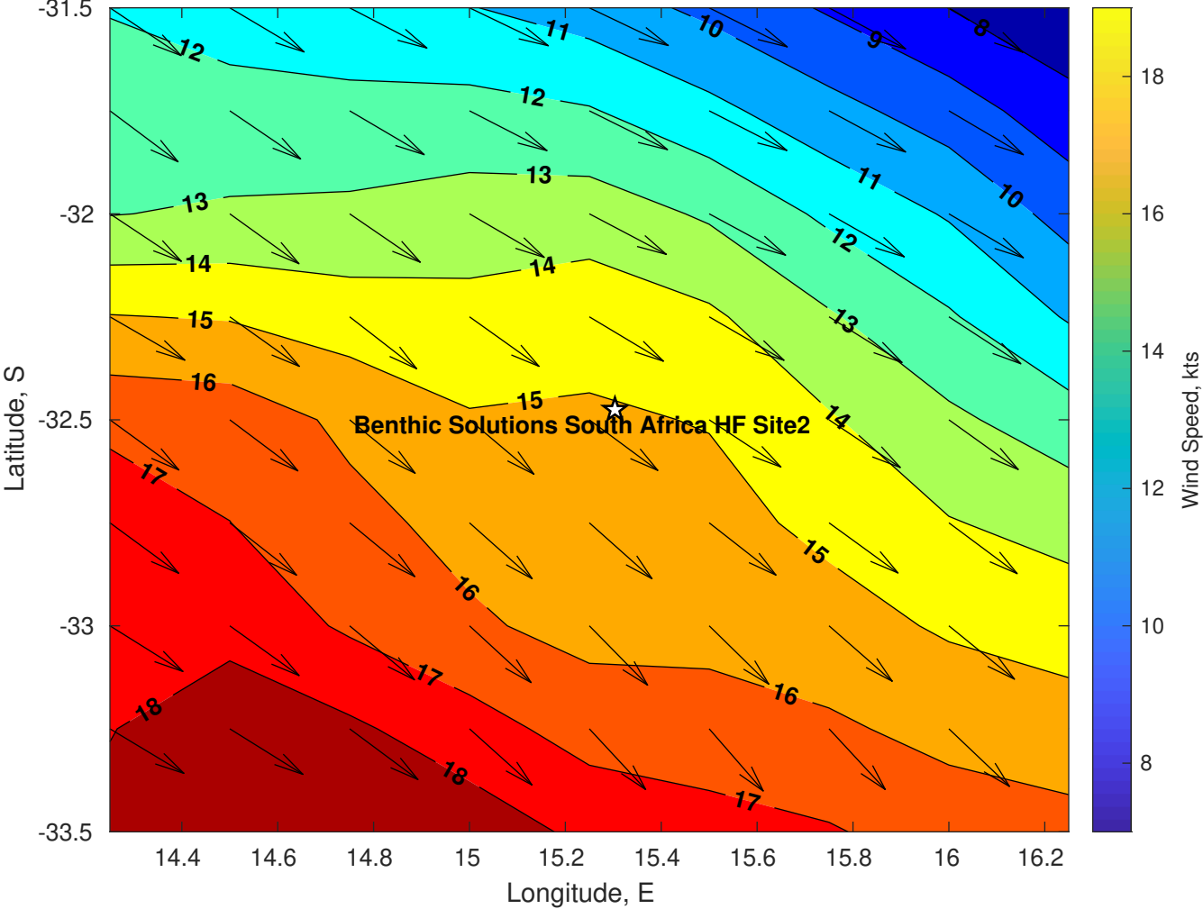
Winds (kts) for Benthic Solutions South Africa HF Site2 at 09-May-2025 09:00:00
