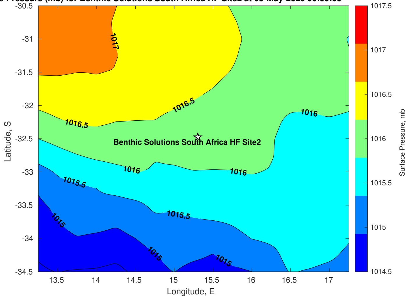
Surface Pressure (mb) for Benthic Solutions South Africa HF Site2 at 09-May-2025 00:00:00
