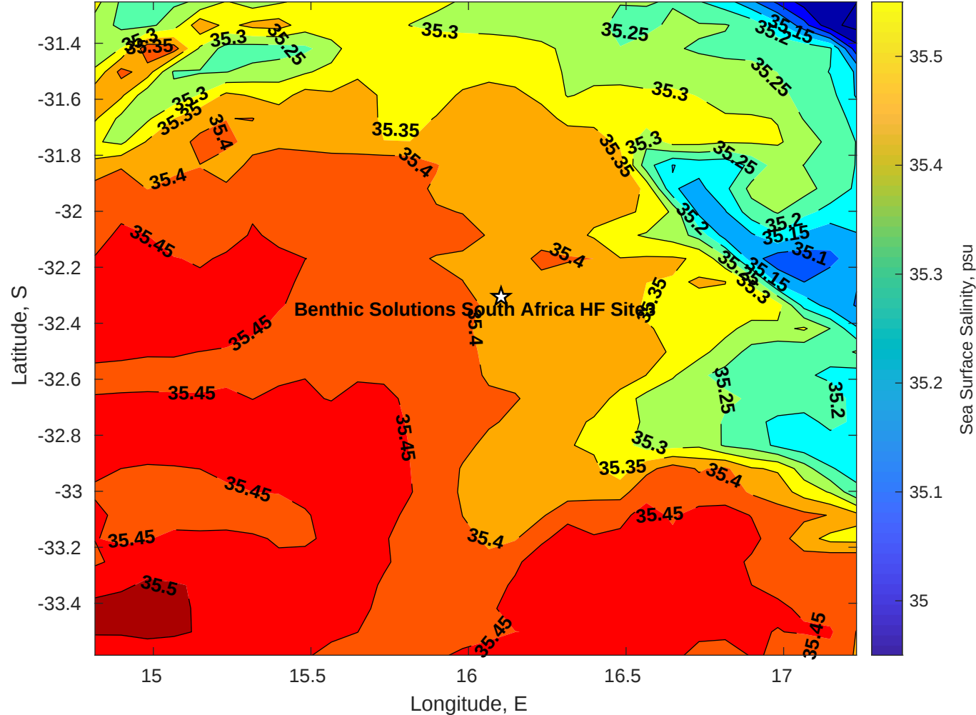
Surface Salinity for Benthic Solutions South Africa HF Site3 at 08-May-2025 00:00:00
