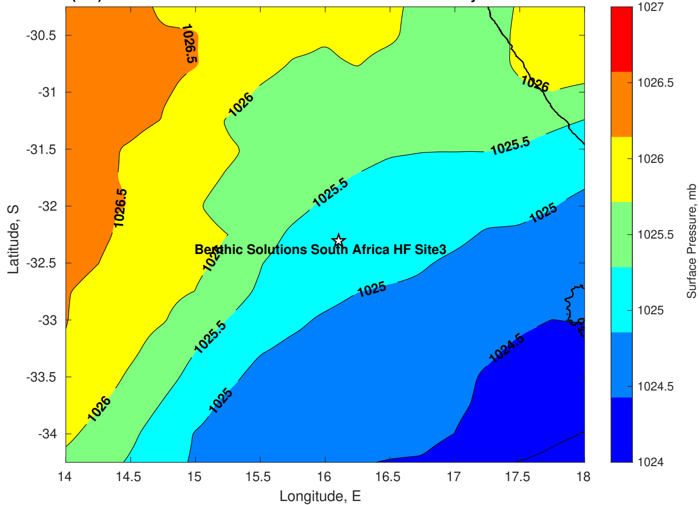
Surface Pressure (mb) for Benthic Solutions South Africa HF Site3 at 11-May-2025 00:00:00
