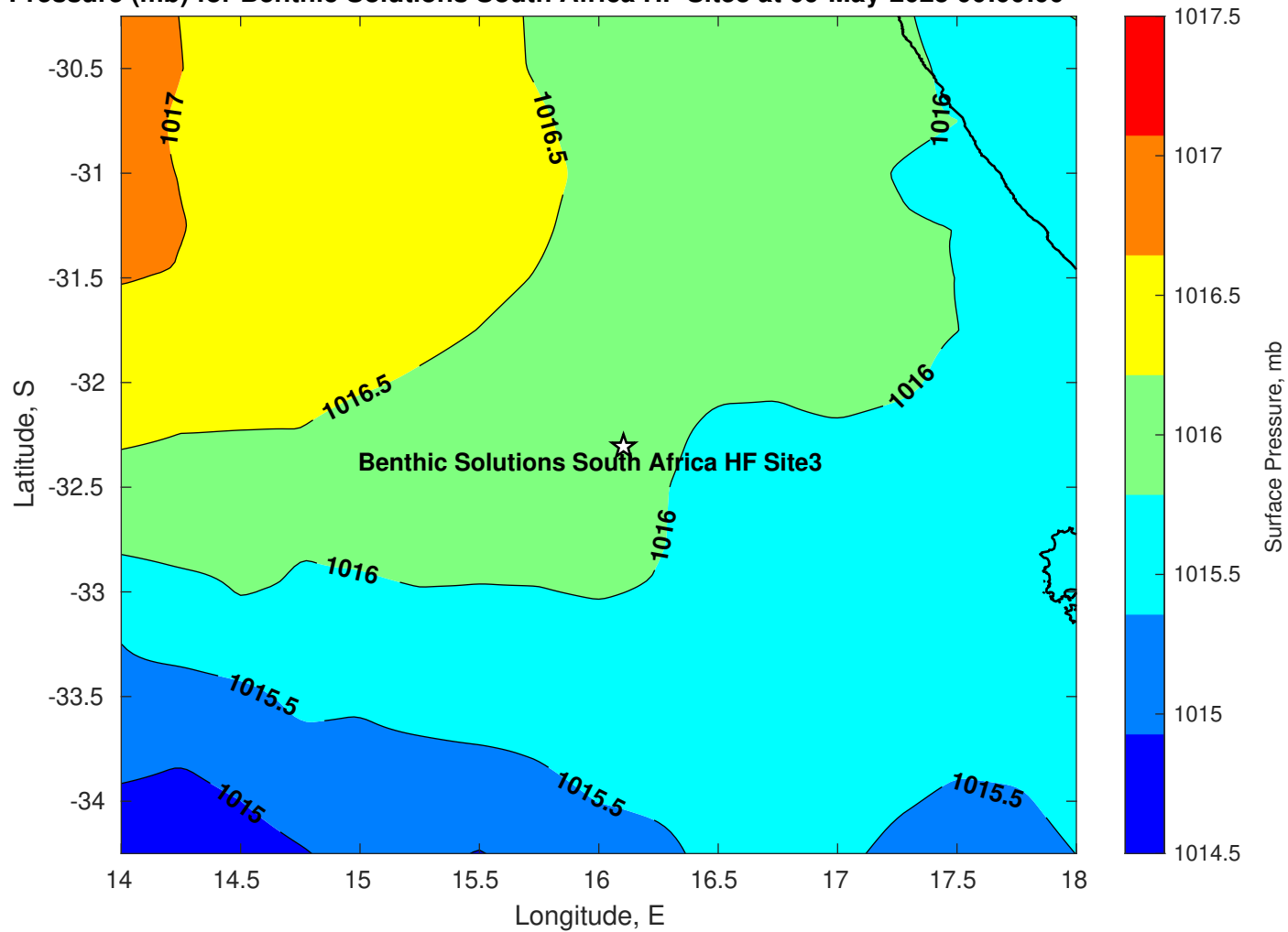
Surface Pressure (mb) for Benthic Solutions South Africa HF Site3 at 09-May-2025 00:00:00
