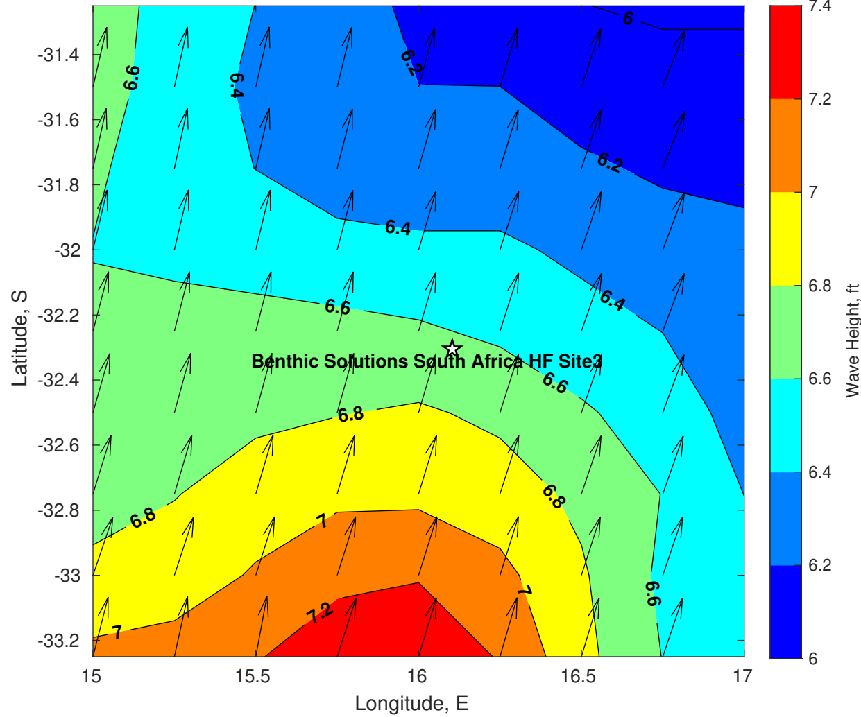
Wave Height (ft) for Benthic Solutions South Africa HF Site3 at 09-May-2025 09:00:00
