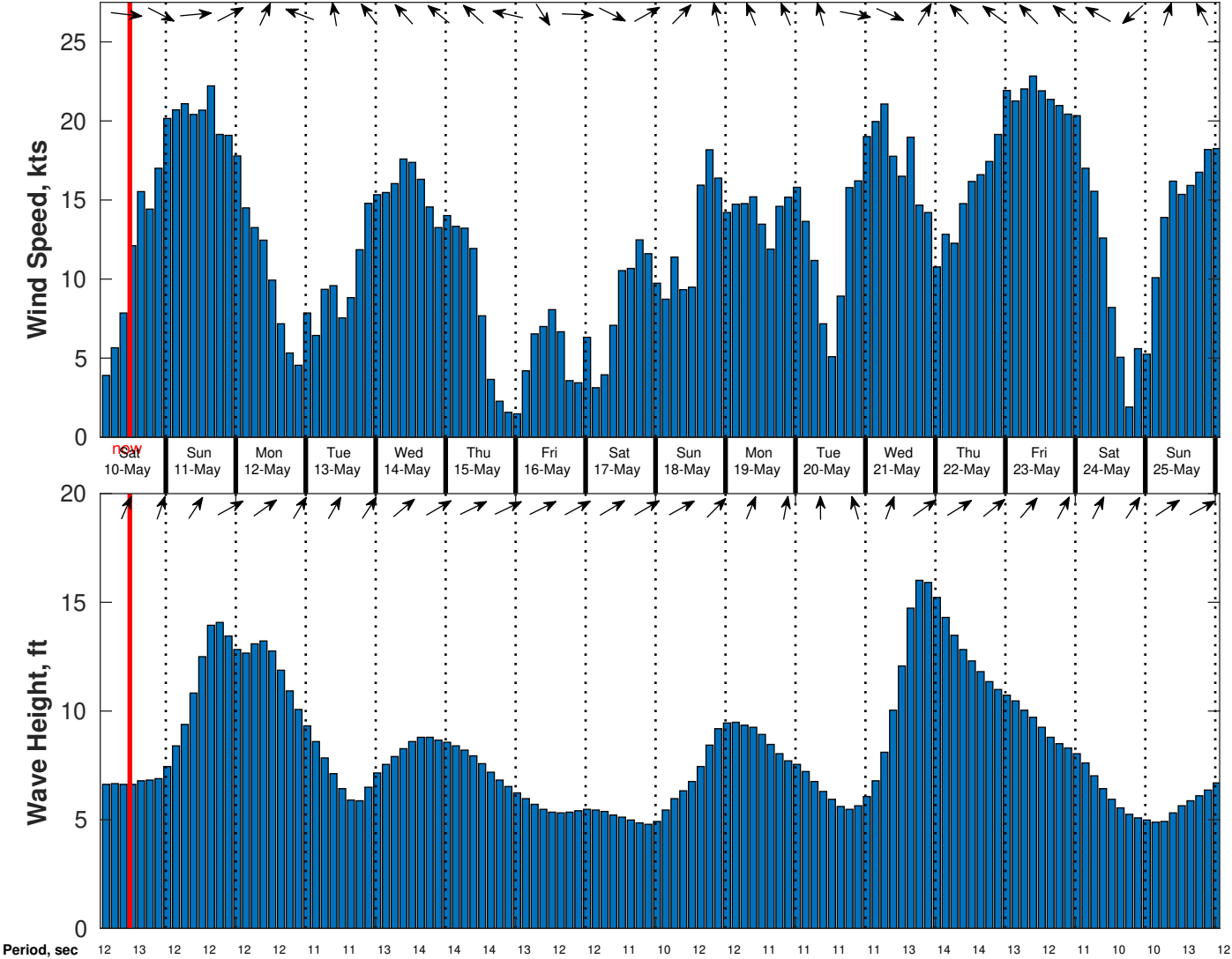
Wind & Wave Forecast for Benthic Solutions South Africa HF Site3 from 09-May-2025 02:00:00 to 25-May-2025 02:00:00
