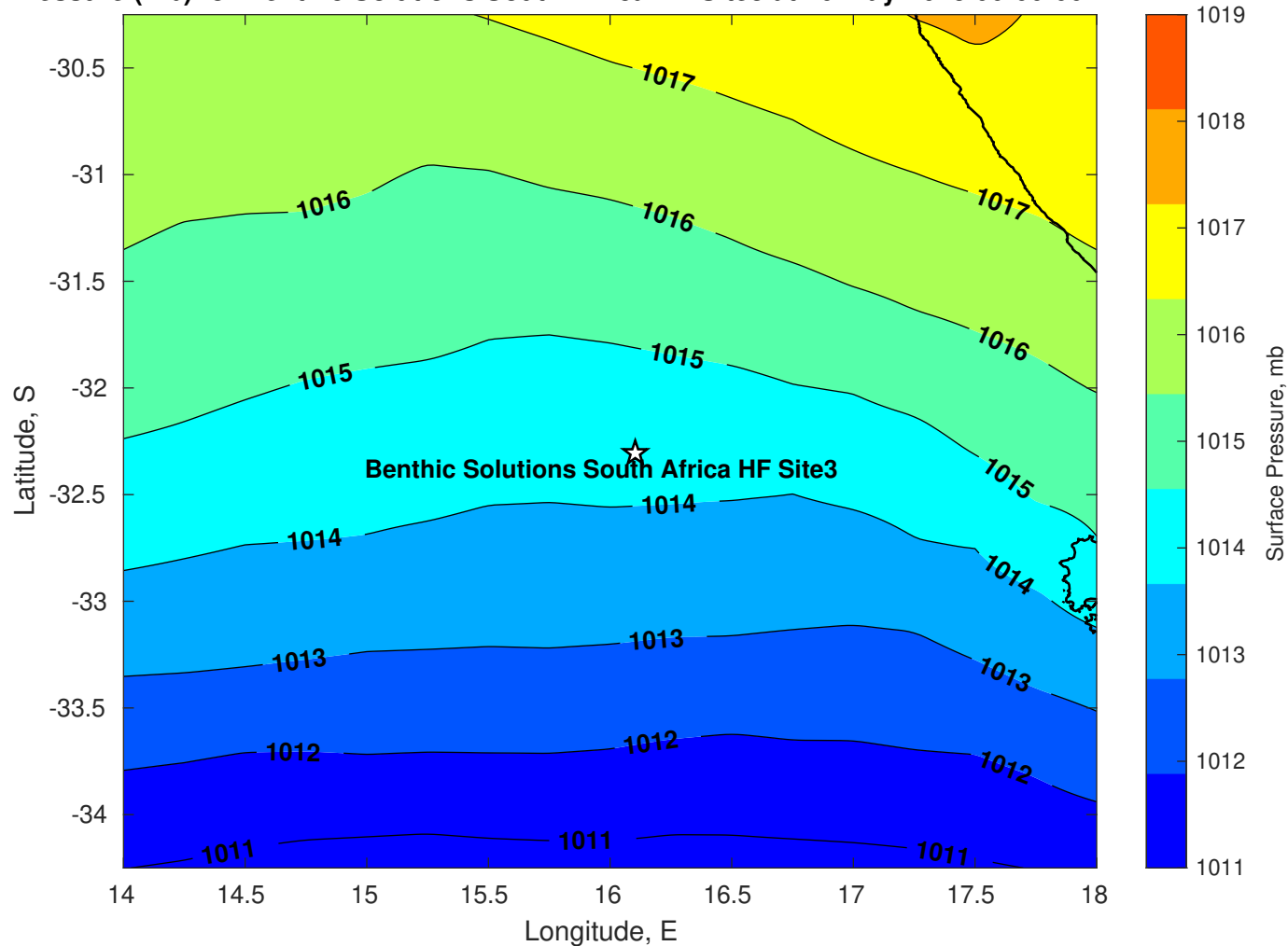
Surface Pressure (mb) for Benthic Solutions South Africa HF Site3 at 10-May-2025 00:00:00
