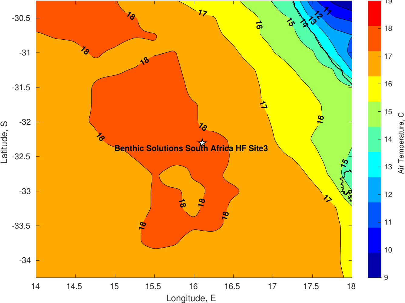
Air Temperature (C) for Benthic Solutions South Africa HF Site3 at 09-May-2025
