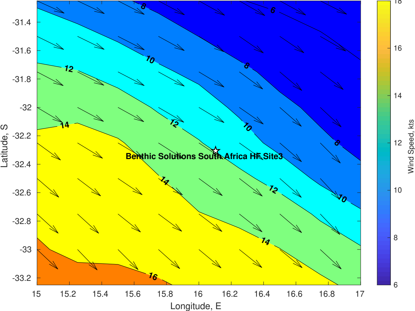
Winds (kts) for Benthic Solutions South Africa HF Site3 at 09-May-2025 09:00:00
