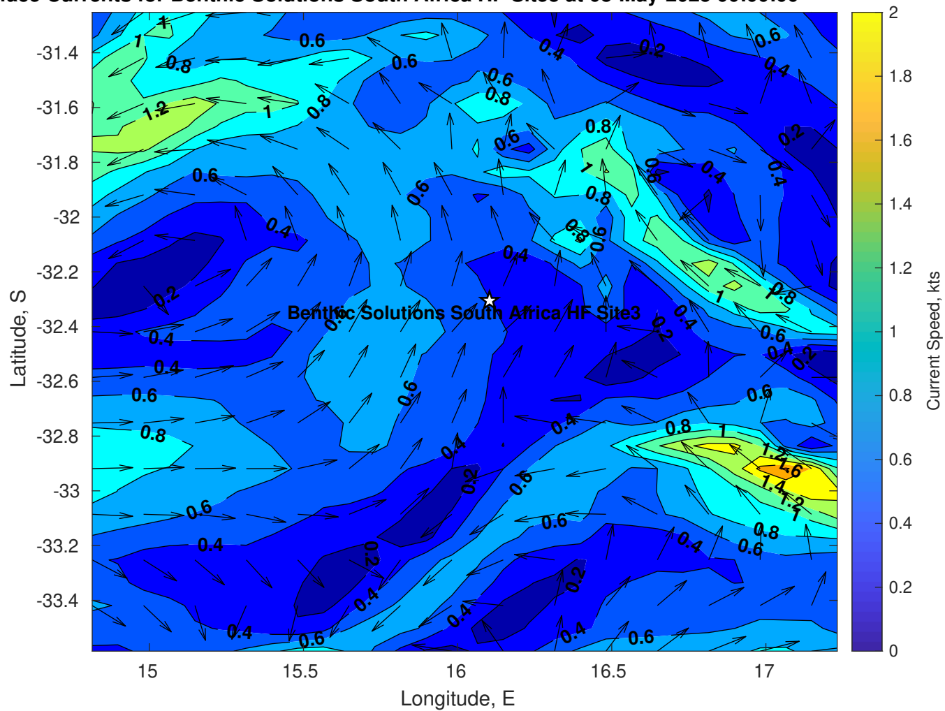
Surface Currents for Benthic Solutions South Africa HF Site3 at 08-May-2025 00:00:00
