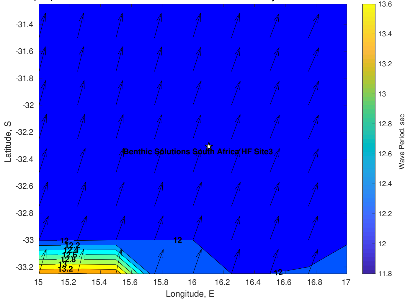
Wave Period (sec) for Benthic Solutions South Africa HF Site3 at 09-May-2025 09:00:00
