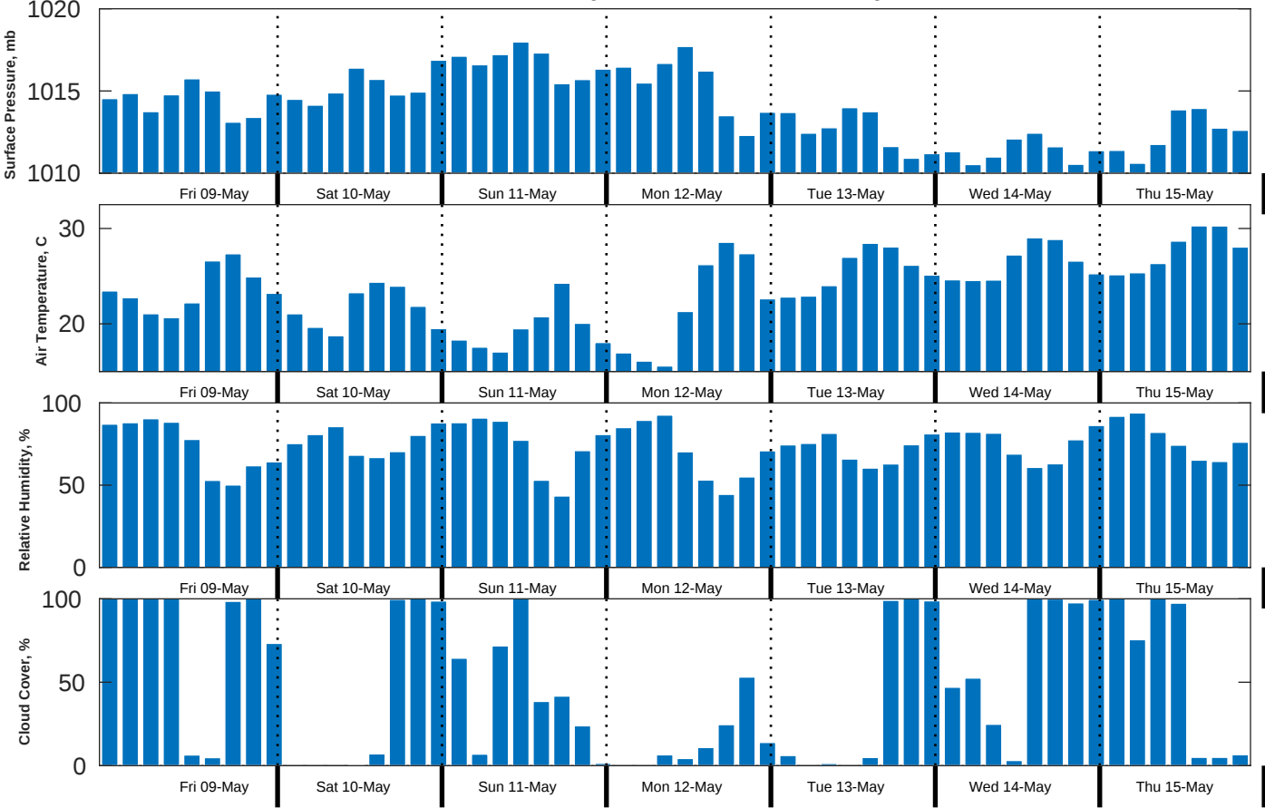
Met Forecast for Brooks McCall from 09-May-2025 00:00:00 to 16-May-2025 00:00:00
