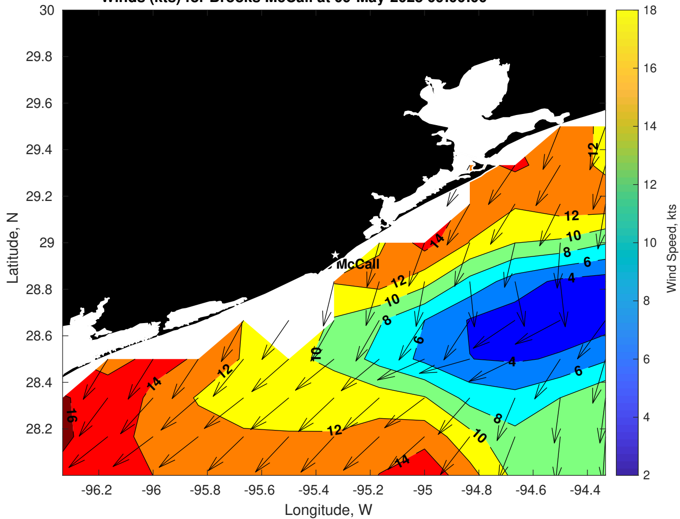
Winds (kts) for Brooks McCall at 09-May-2025 09:00:00
