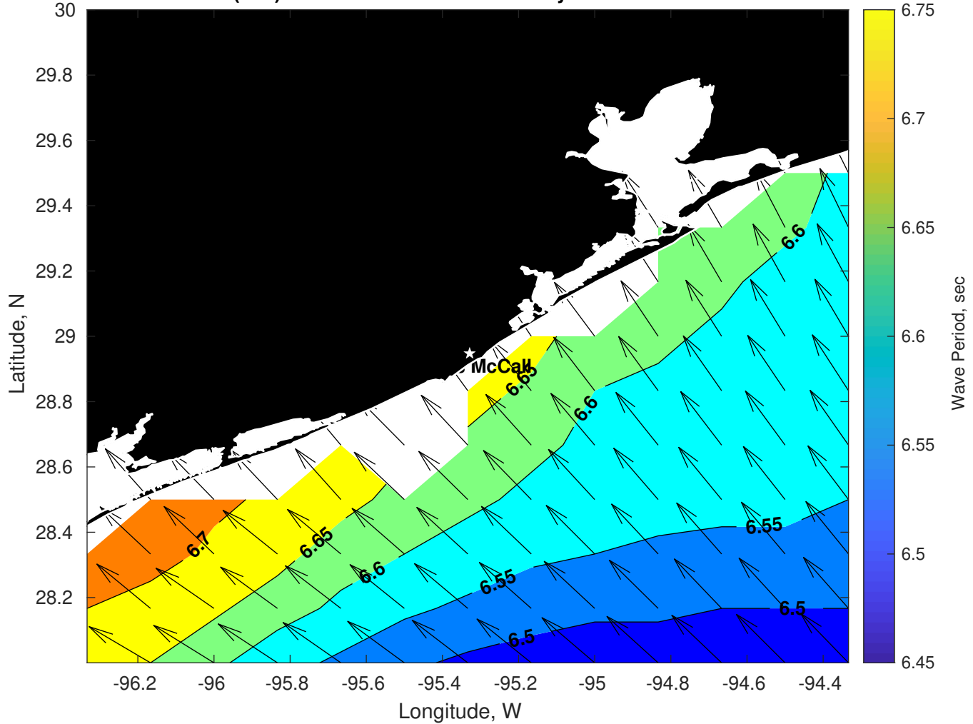
Wave Period (sec) for Brooks McCall at 09-May-2025 09:00:00
