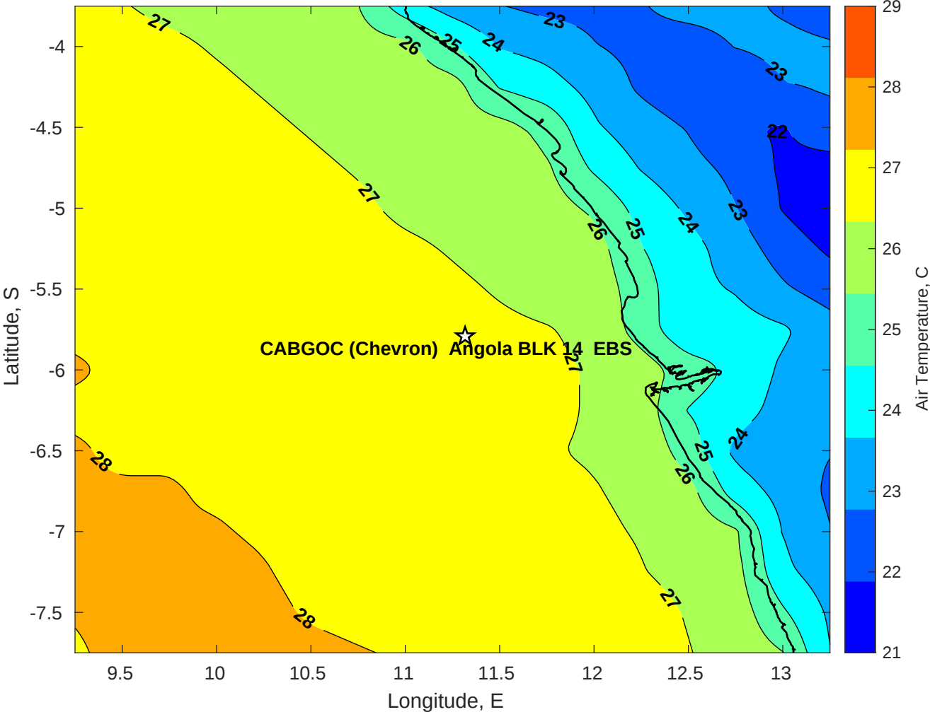
Air Temperature (C) for CABGOC (Chevron) Angola BLK 14 EBS at 09-May-2025
